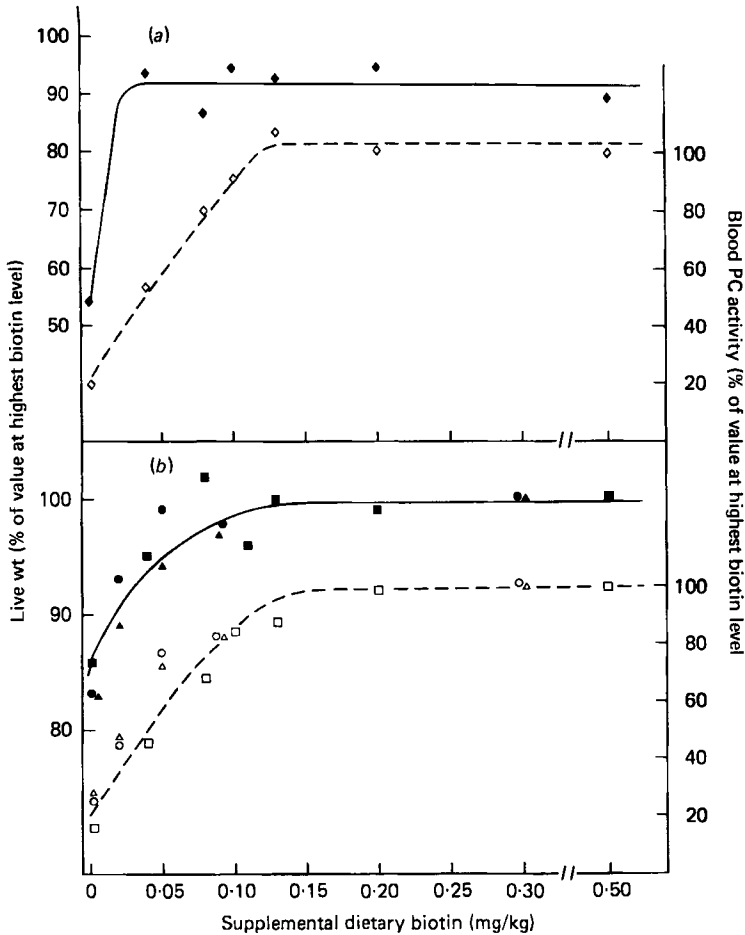
Fig. 1. Expts 1, 2 and 3. Responses of blood pyruvate carboxylase (pyruvate: carbon dioxide ligase (ADP-forming), EC 6.4.1.1; PC) activity (---) and live weight (—) to different levels of supplemental dietary biotin in broilers at 5 weeks of age. (○, △, □), PC; (●, ▲, ■), live weight for males (○, ●) and females (△, ▲) in Expt 1 and males (□, ■) in Expt 2 ( b ; large scale). PC (◇) and live weight (◆) are for males in Expt 3 ( a ; small scale). At each biotin level, PC in Expts 1, 2 and 3 and live weight in Expts 1 and 2 are expressed as percentages of the value at the highest biotin level for that sex in that experiment; live weight in Expt 3 is expressed as the percentage of the mean live weight of males given the highest biotin levels in Expts 1 and 2. The curves are fitted by eye.
