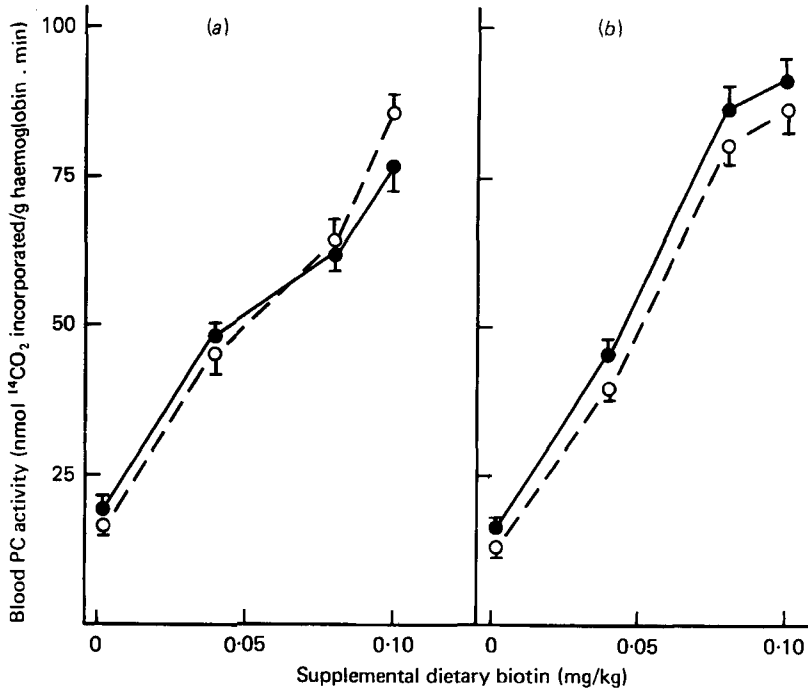
Fig. 2. Expt 2. Blood pyruvate carboxylase (pyruvate: carbon dioxide ligase (ADP-forming), EC 6.4.1.1; PC) activity at (a) 3 and (b) 7 weeks of age in broilers housed in pens with floors of wire mesh (○—○) or wood shavings (●—●) and fed on diets containing different levels of supplemental biotin. Mean values with their standard errors represented by vertical bars.
