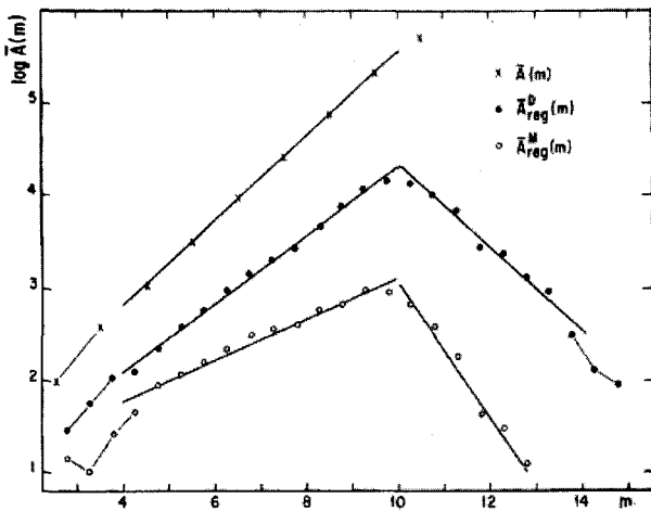
Fig. 2. The number of double stars (middle lines) and multiple stars (bottom lines) are plotted as a function of apparent visual magnitudes, m . The top line shows the number of single field stars. The symbols represent the observational data, and the lines are least-squares fits. These show incompleteness starting at magnitude 10. (Reprinted from ApJ, 258, 589, 1982.)
