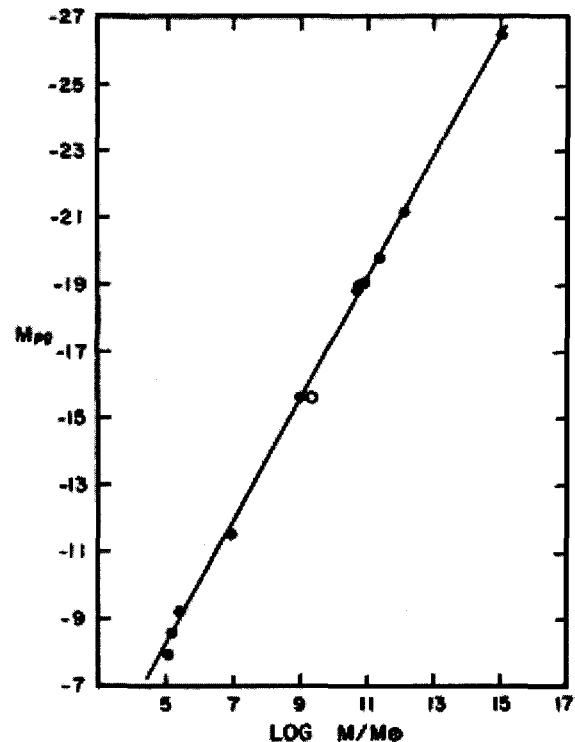
Fig. 1. Poveda found that for spherical systems from globular clusters to clusters of galaxies the relationship between their photographic absolute magnitudes (ordinates) and the logarithms of their masses in solar units (abscissae) is a linear one. (Reprinted from ApJ, 134, 910, 1961.)
