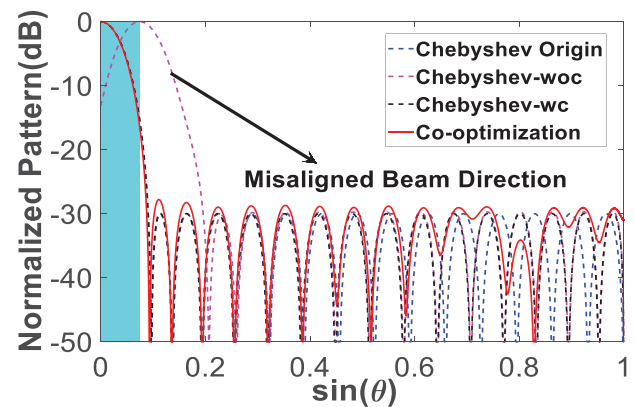
Figure 3. Performance comparison with z_{\max}(P) = \lambda .
