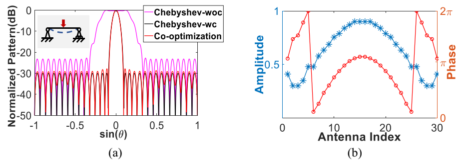
Figure 6. Pattern and excitations: (a) normalized pattern and (b) excitations.
