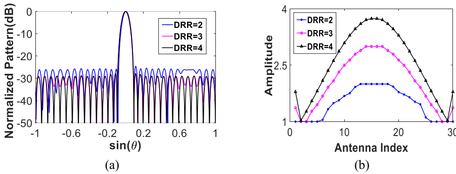
Figure 2. Results of the array antenna without deformation under different DRR: (a) normalized pattern and (b) amplitude excitation.
