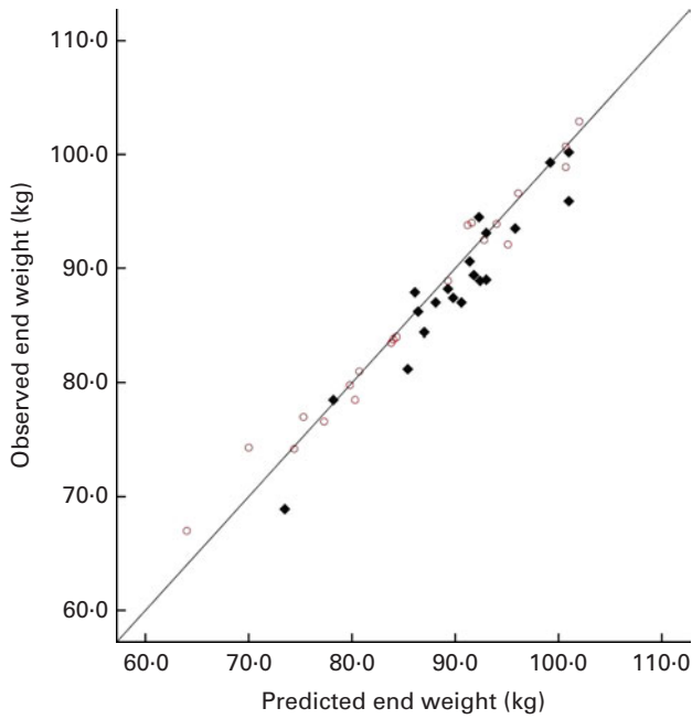
Fig. 1. Predicted body weight (National Institute of Diabetes and Digestive and Kidney Diseases (NIDDK) model) and observed weight at the end of the experiment. Drinks given over 28 d: ◆, sucrose; ○, aspartame. (A colour version of this figure can be found online at http://www.journals.cambridge.org/bjn )
