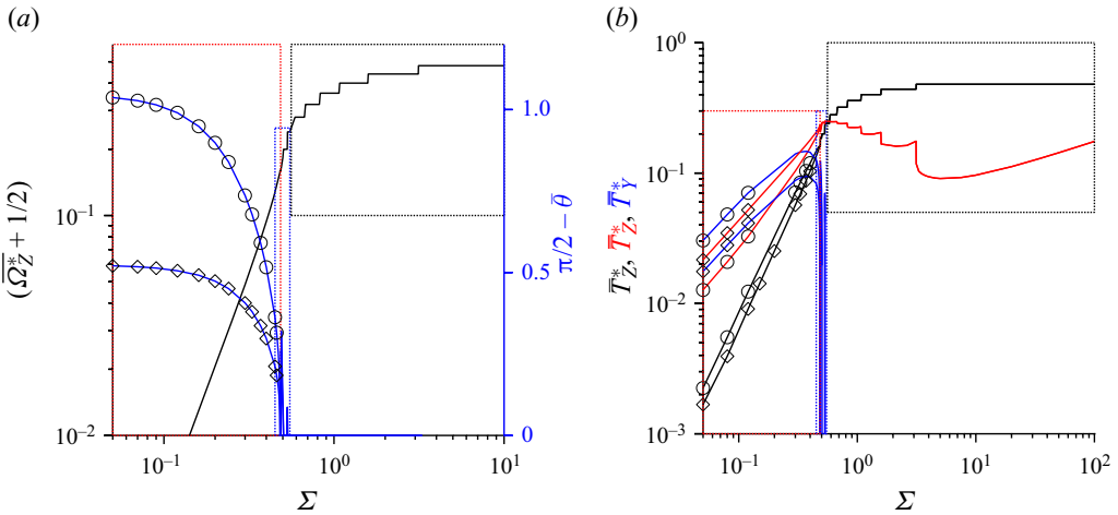
Figure 4. The variation in (a) (\bar{\Omega}_Z^* + \frac{1}{2}) (black line) and \pi/2 - \bar{\theta} (blue line) and (b) \bar{T}_Z^* (black line), \bar{T}_Z^* (red line) and \bar{T}_Y^* (blue line) with the parameter \Sigma for \omega^* = 0.02 . The red, black and blue rectangles are expanded in figures 6, 10 and 12, respectively. Detailed analyses of the dynamics for the parameter regimes in the red, black and blue rectangles are carried out in §§ 5.1.1, 5.1.2 and 5.1.3, respectively. The initial conditions are \phi = 0 and \theta = (\pi/3) ( \circ ) and \theta = (\pi/6) ( \diamond ).
