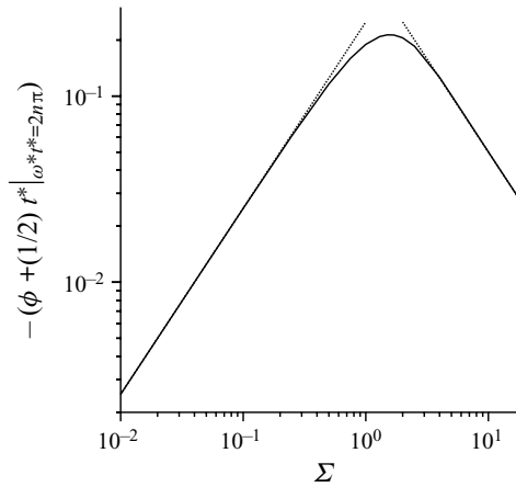
Figure 21. The variation of -\left(\phi + \frac{1}{2}t^*\right)_{\omega^*t^*=2n\pi} with the parameter \Sigma for \omega^* = 0.5 . The dashed black line on the left is the analytical result \frac{1}{4}\Sigma consistent with (4.20) and the dashed black line on the right is 0.5/\Sigma .
