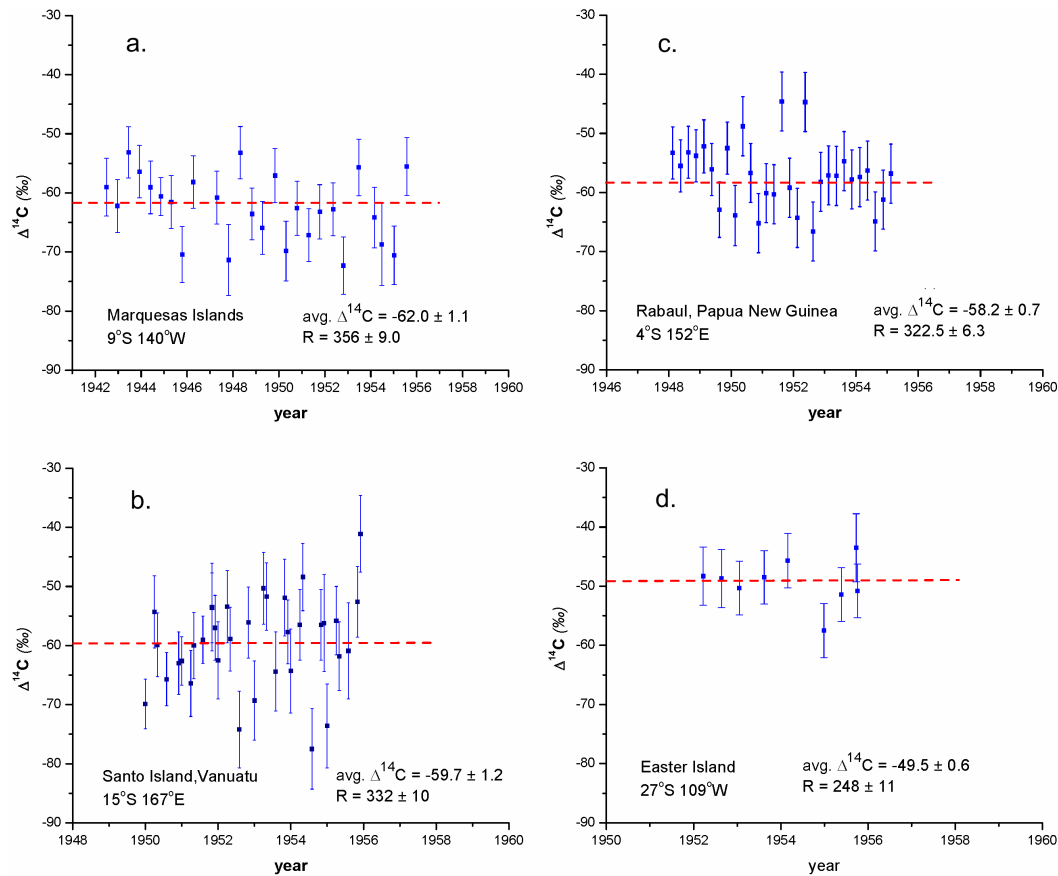
Figure 3 South Pacific coral \Delta^{14}\text{C} time series for the 4 sites studied: a) Marquesas Islands; b) Espiritu Santo Island, Vanuatu; c) Rabaul, Papua New Guinea; d) Ovahe, Easter Island. Reservoir ages ( R ) are taken as the weighted average of the measurements. Uncertainties are 1\sigma , taken as the external variance from the sample distribution.
