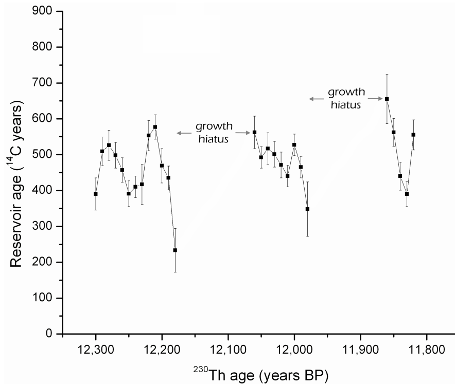
Figure 5 Plot of the surface ocean reservoir age at Vanuatu between 11.9 and 12.3 cal kyr BP. Data compiled from Burr et al. (1998) and Friedrich et al. (2004). The ^{230}\text{Th} ages from Burr et al. have been recalculated using the half-life values of Cheng et al. (2000). Uncertainties are 1\sigma .
