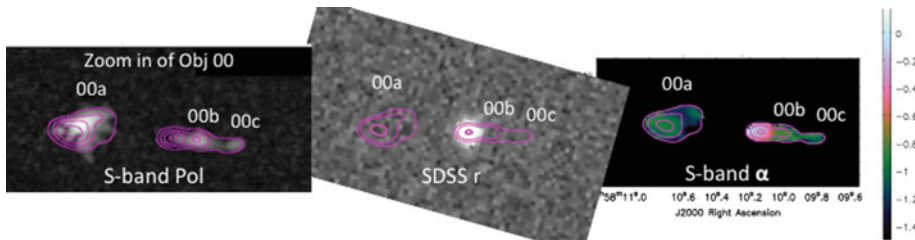
Figure 2. Three zoomed in images of a control source. In each zoom-in the contours trace the total intensity of the VLA observations integrated across the entire S-band (RMS= 20\mu\text{Jy} ), 2-4GHz. The left image shows the polarization in greyscale. The middle image shows the SDSS r-band image in greyscale, and the right image shows the spectral index, \alpha where S_\nu \propto \nu^\alpha , as described by the colorbar.
