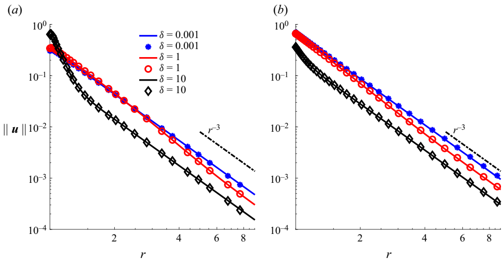
Figure 3. Velocity magnitude \|\mathbf{u}\| = \sqrt{u^2 + v^2} as a function of the distance from the squirmer’s surface for (a) \theta = 0 and (b) \theta\pi/2 . In both panels, b = 1.025 and \lambda = 10 . The solid curves are obtained from the N-B model and the symbols denote numerical simulations.
