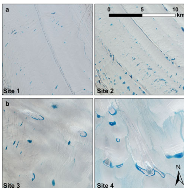
Fig. 8. A comparison of SGLs on the (a) floating tongue (Sites 1 and 2) and (b) grounded region (Sites 3 and 4) of Petermann Glacier in pansharpended OLI images. Sites 1–4 are located at increasingly up-glacier positions, as indicated in Figure 1, and the images were captured on 27 June 2014 for Site 1, and 30 June 2014 for Sites 2–4.
