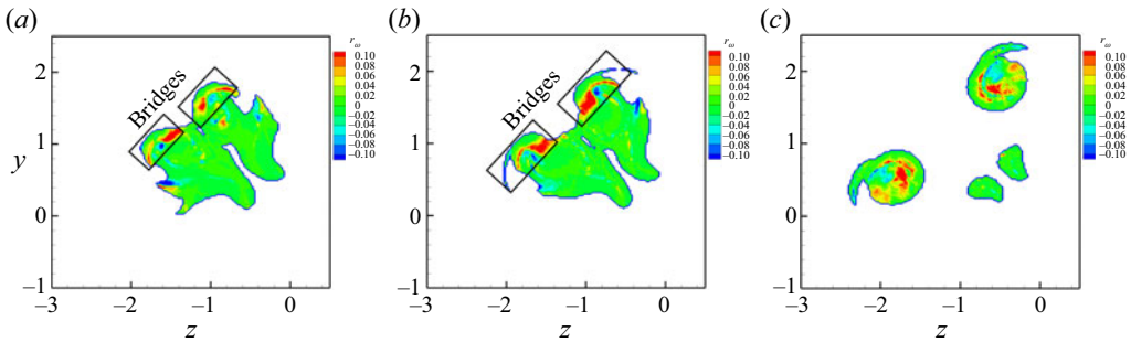
Figure 21. The r_\omega contours in the dividing plane at t = (a) 5.16, (b) 5.28 and (c) 6. Contours are only shown in regions wherein |\omega| > 0.4\omega_0 .
