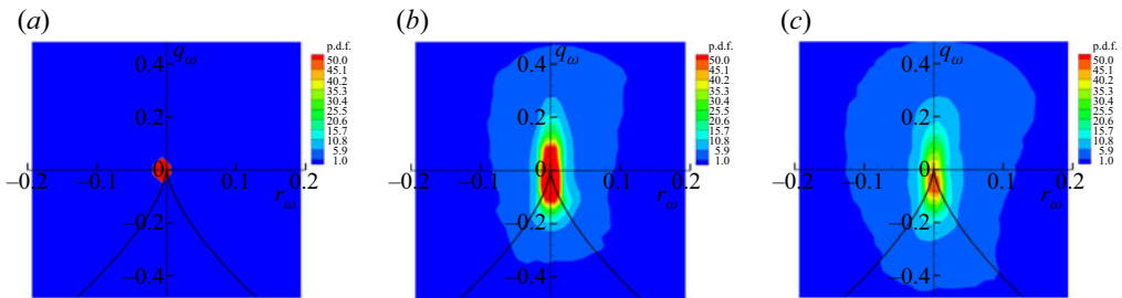
Figure 22. The q_\omega – r_\omega joint p.d.f. filled contours t = (a) 0, (b) 5.16 and (c) 6. Only points with |\omega| > 0.4\omega_0 are considered.
