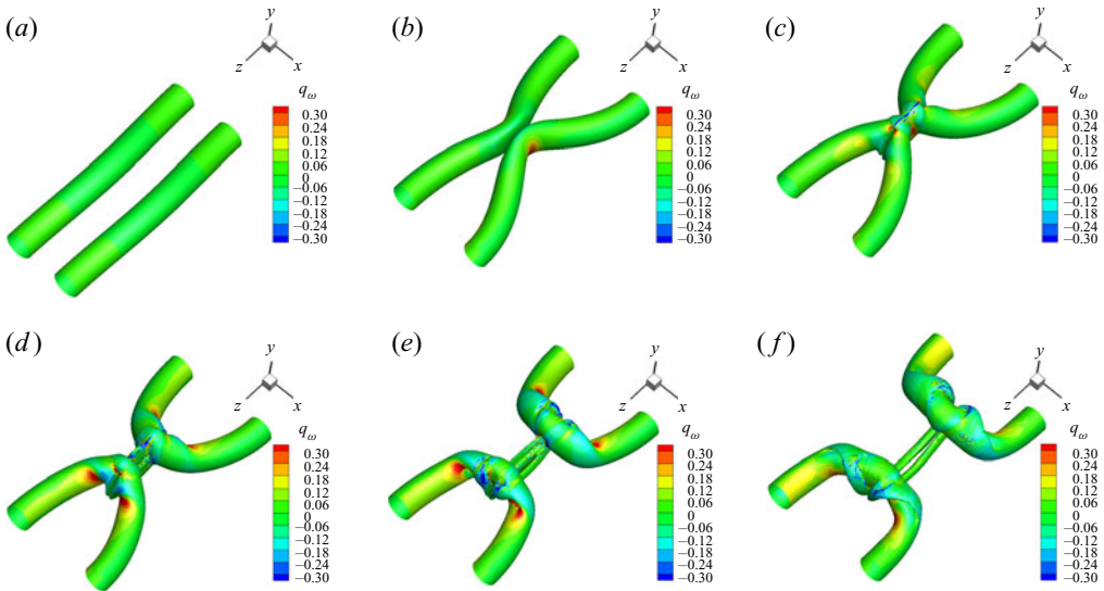
Figure 15. The |\omega| isosurfaces at 30% of maximum initial vorticity coloured by q_\omega at t = (a) 0, (b) 3.6, (c) 4.4, (d) 4.8, (e) 5.4 and (f) 6 .
