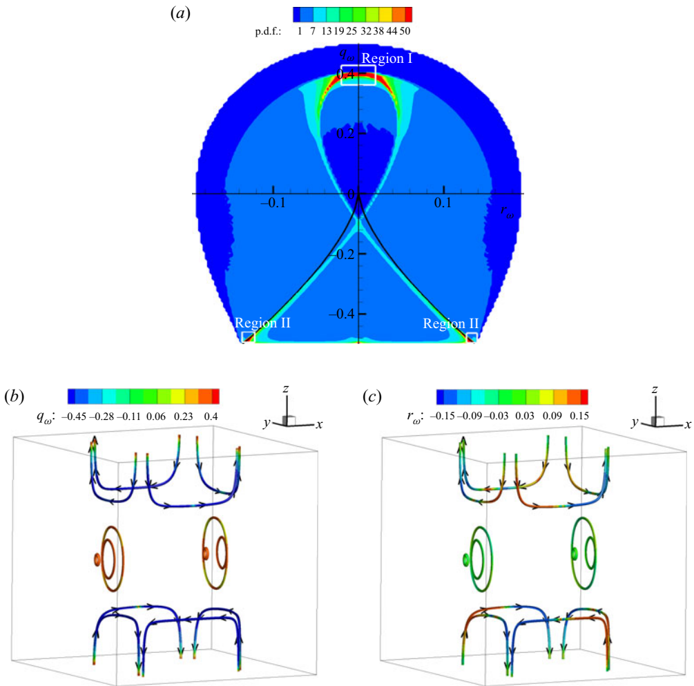
Figure 12. (a) Filled contour plot of the q_\omega – r_\omega joint p.d.f. for the initial field of a Taylor–Green vortex flow. Field vortex lines in physical space dominated by regions I and II of the q_\omega – r_\omega joint p.d.f. coloured by (b) q_\omega (c) r_\omega .
