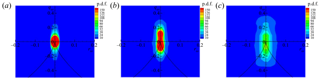
Figure 18. The q_\omega – r_\omega joint p.d.f. filled contours at t = (a) 0, (b) 4.4 and (c) 6. Only points with |\omega| > 0.3\omega_0 are considered.
