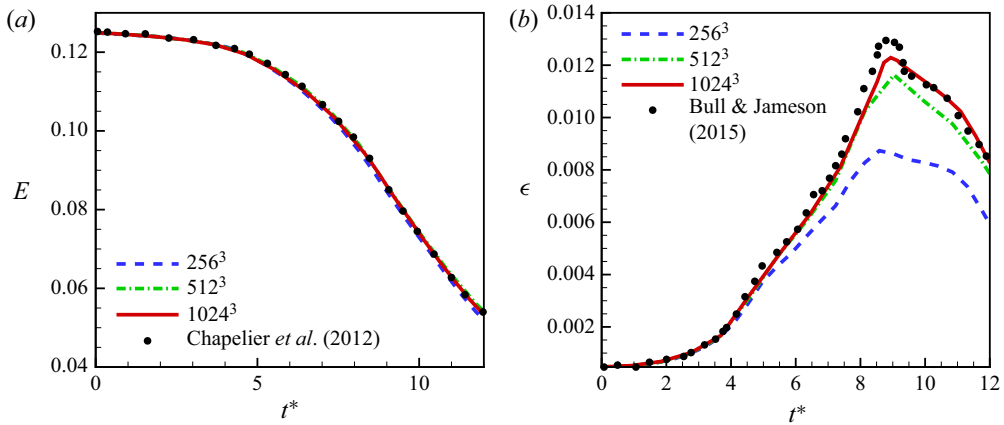
Figure 3. Time evolution of (a) normalized kinetic energy ( E/U_0^2 ) and (b) normalized mean dissipation rate ( \epsilon/(U_0^3/L) ) for a Taylor–Green vortex.
