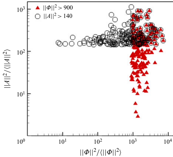
Figure 10. Scatter plot for extreme values of \|\Phi\|^2 (> 900) and \|A\|^2 (> 140) for Re_\lambda = 225 .
