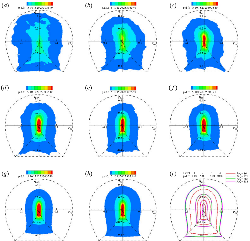
Figure 8. The q_{\omega} - r_{\omega} joint p.d.f. filled contour plots for Re_{\lambda} = (a) 1, (b) 6, (c) 9, (d) 14, (e) 18, (f) 25, (g) 86 and (h) 225; (i) line contour plots for Re_{\lambda} = 86 –588.
