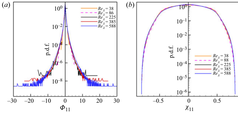
Figure 7. Marginal p.d.f. of the longitudinal component of the (a) un-normalized ( \Phi_{11} ) and (b) normalized ( \chi_{11} ) vorticity gradient tensor.
