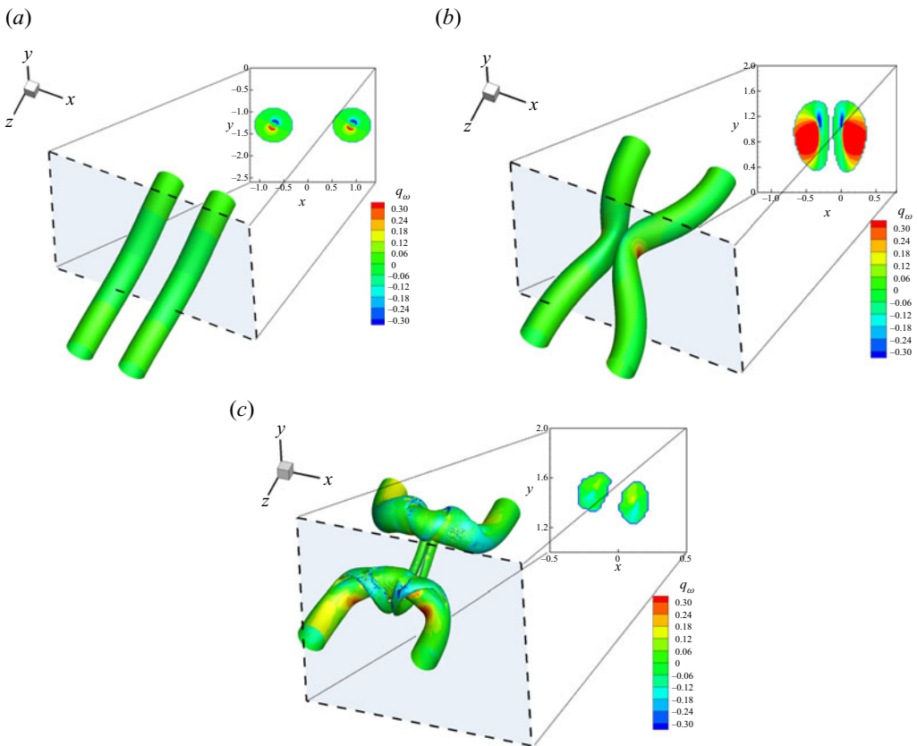
Figure 16. The q_\omega contours in the symmetry plane at t = (a) 0, (b) 3.6 and (c) 6 . Contours are only shown in regions wherein |\omega| > 0.3\omega_0 .
