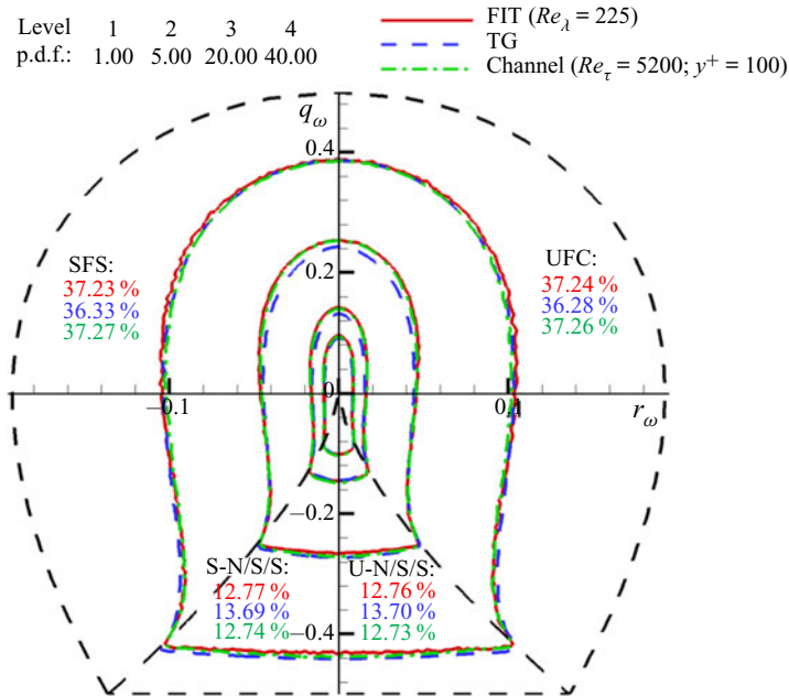
Figure 14. The q_\omega - r_\omega joint p.d.f. line contour plots and population fractions of non-degenerate topologies for forced isotropic turbulence (FIT) at Re_\lambda = 225 , Taylor–Green vortex flow (TG) at t^* = 12 (shortly after peak dissipation) and turbulent channel flow at Re_\tau = 5200 on the wall-normal plane y^+ = 100 . Data for the turbulent channel flow case are obtained from Johns Hopkins Turbulence Database (Moser, Kim & Mansour 1999; Perlman et al. 2007; Li et al. 2008).
