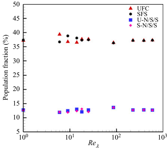
Figure 9. Population fraction of non-degenerate vortex line topologies for forced isotropic turbulence at different Re_\lambda .
