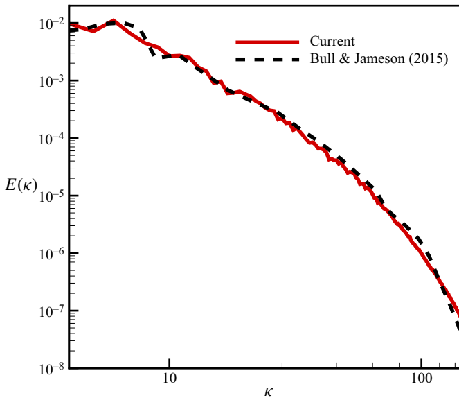
Figure 4. Kinetic energy spectrum just after peak dissipation at t^* = 9 .
