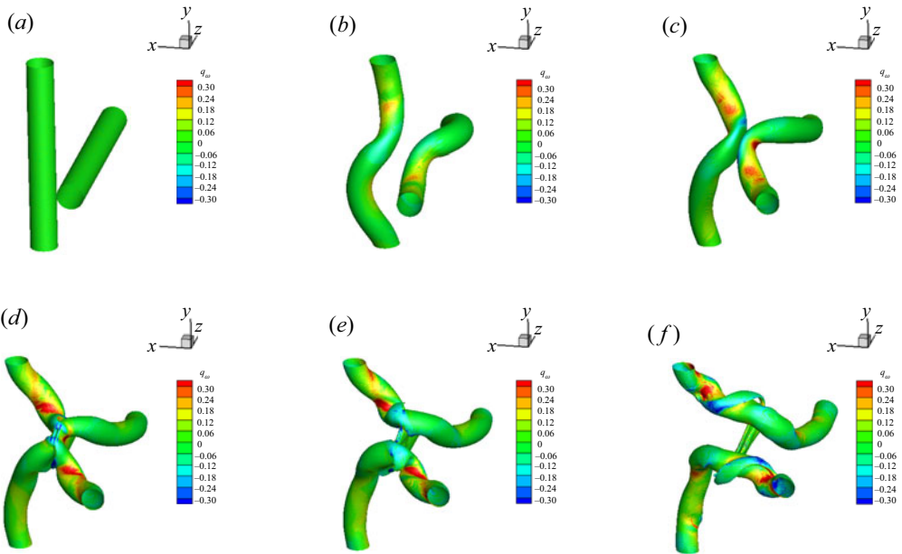
Figure 19. The |\omega| isosurfaces at 40% of maximum initial vorticity coloured by q_\omega at t = (a) 0, (b) 2.64, (c) 4.32, (d) 4.92, (e) 5.28 and (f) 6 .
