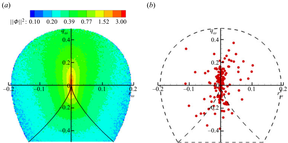
Figure 11. (a) Conditional average of the Frobenius norm of the vorticity gradient tensor ( \langle \Phi^2 | r_\omega, q_\omega \rangle / \langle \Phi^2 \rangle ) in the q_\omega-r_\omega plane for Re_\lambda = 225 ; (b) scatter plot of extreme vorticity magnitude ( \|\Phi\|^2 > 1000 ) in the q_\omega-r_\omega plane.
