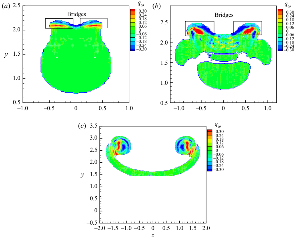
Figure 17. The q_\omega contours in the dividing plane at t = (a) 4.4, (b) 4.8 and (c) 6. Contours are only shown in regions wherein |\omega| > 0.3\omega_0 .
