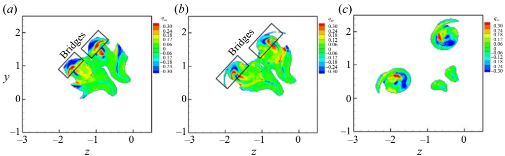
Figure 20. The q_\omega contours in the dividing plane at t = (a) 5.16, (b) 5.28 and (c) 6 . Contours are only shown in regions wherein |\omega| > 0.4\omega_0 .
