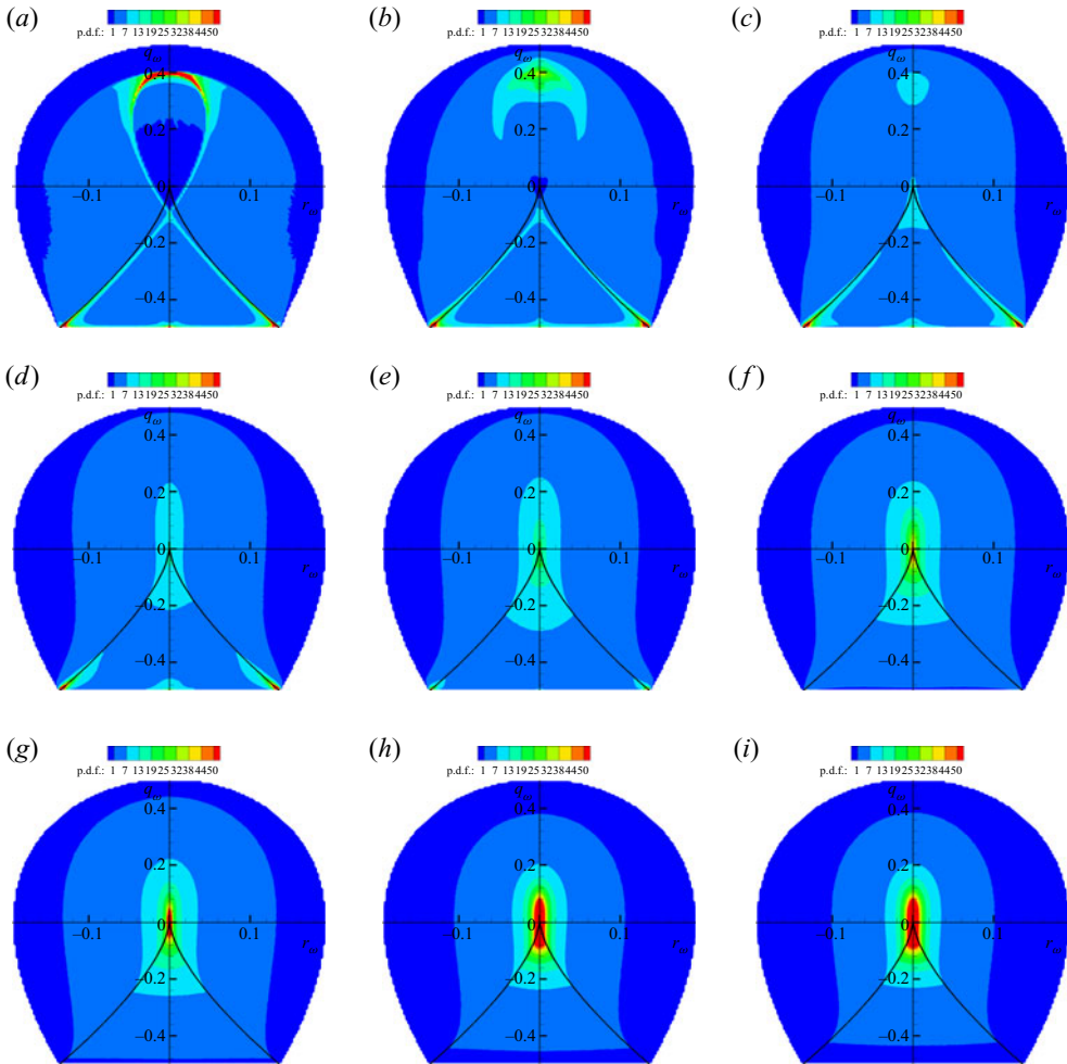
Figure 13. The q_\omega - r_\omega joint p.d.f. filled contour plots for Taylor–Green vortex simulation at (a) t^* = 0 , (b) t^* = 0.132 , (c) t^* = 0.145 , (d) t^* = 0.160 , (e) t^* = 0.185 , (f) t^* = 0.740 , (g) t^* = 5 , (h) t^* = 9.23 and (i) t^* = 11.57 .
