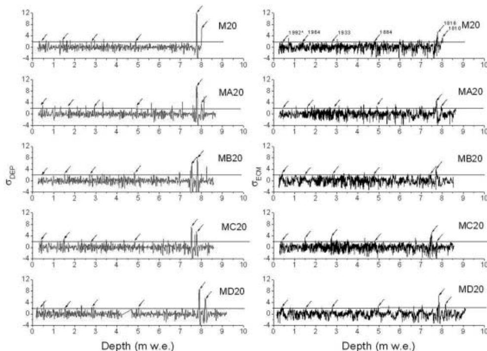
Fig. 3. ECM (right) and DEP (left) data from the firm cores. The data are normalized to one standard deviation. Peaks exceeding a 2\sigma threshold are considered to be of volcanic origin. Six volcanic peaks were identified in each core and used for dating. These peaks are listed in Table 5. Depth of peak is derived from the snow pits.
