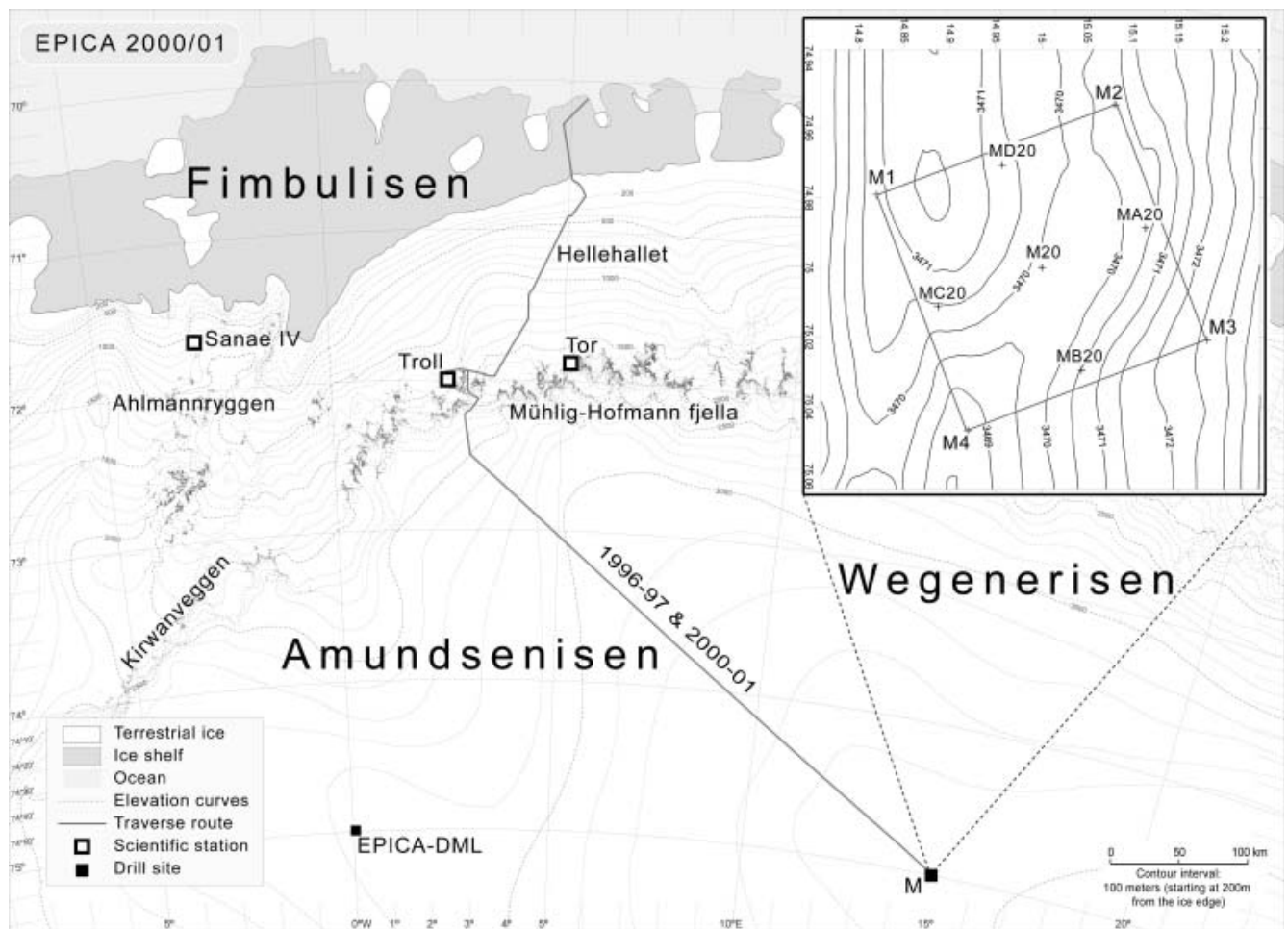
Fig. 1. The study area in DML, with the traverse route used in 1996/97 and 2000/01. The insert map shows drill locations (M20, MA20, MB20, MC20 and MD20) and the surface topography as measured by kinematic global positioning system (GPS) in the box limited by points M1–M4. The medium-depth core mentioned in the text was drilled \sim 5 m from M20. The EPICA-DML core site where a deep core is currently being drilled is also marked.
