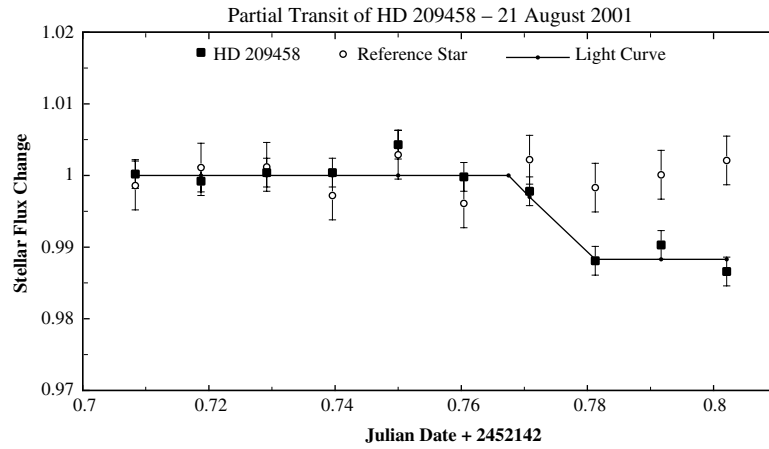
Figure 2 The egress of the planetary transit on 21 August 2001.
