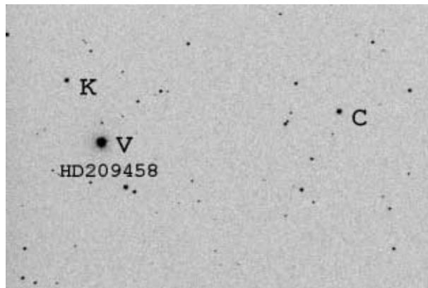
Figure 1 Sample data image of the field around HD 209458 (V; m_v = 7.65 ) showing the comparison star (C = TYC 1688-1766-1; m_v = 10.13 ) and check star (K = GSC 1688-1716; m_v = 11.62 ) which are typically used in differential photometry to assure data quality.
