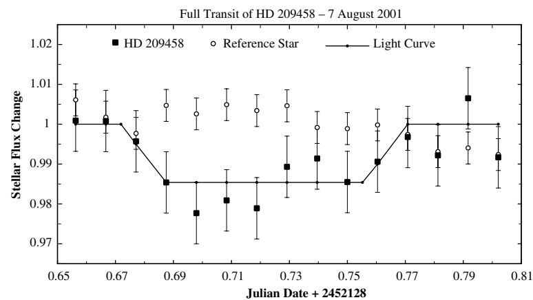
Figure 4 A complete transit of the planet orbiting HD 209458 observed on 7 August 2001. The slope of the light curve at ingress and egress was outside the resolution of direct detection, but was calculated from the planet diameter determined by this study. The consistently larger error of the target star versus the check star in this particular transit is unexplained.
