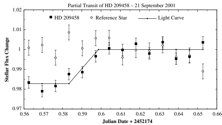
Figure 3 The ingress of the planetary transit of 21 September 2001.
