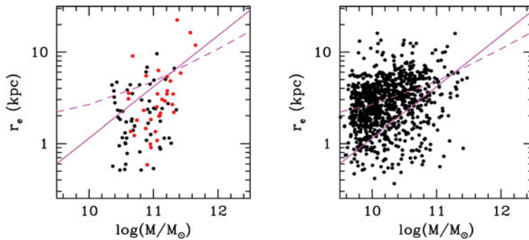
Figure 3. The half-light radius versus the Stellar mass for the passive ( left panel ) and star-forming BzKs galaxies ( right panel ). The magenta lines that are overplotted are the stellar mass relation for the early-type galaxies ( solid line ) and late-type galaxies ( dashed line ) at z \sim 0.1 from the SDSS (Shen et al. 2003).
