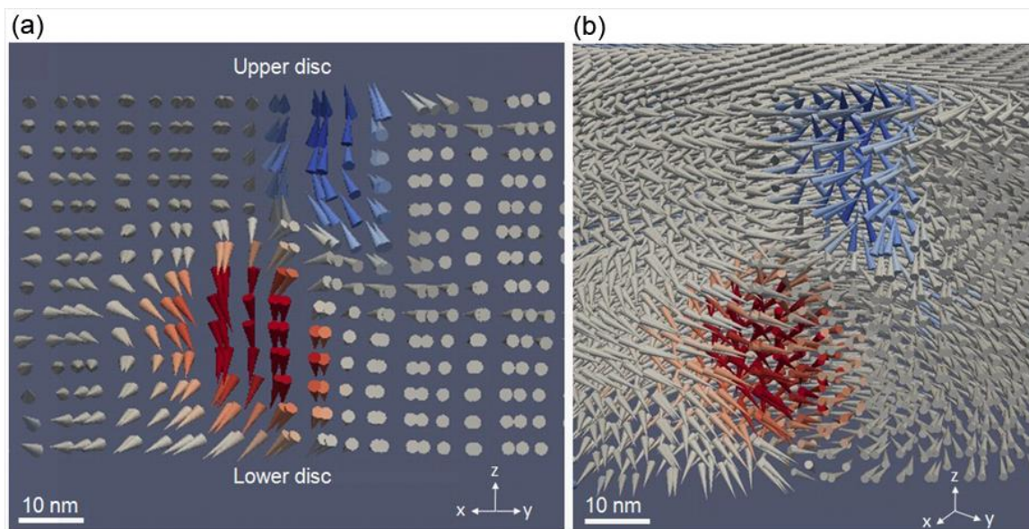
Figure 2. Three-dimensional (3D) view of the reconstructed magnetic vortex cores. The z -directional components are indicated by blue (+ z ) or red ( -z ). (a) The cross-sectional magnetic vectors. The magnetic vectors for the upper and lower vortex cores had opposite z directions. (b) 3D view of the tail-to-tail vortex cores.
