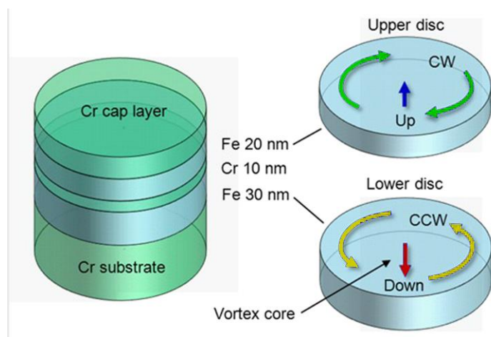
Figure 1. Schematic diagrams of stacked ferromagnetic discs and axes used for 360° observations. Two Fe discs (light blue) with thicknesses of 20 nm (upper) and 30 nm (lower) were separated by a 10 nm Cr disk (green). The direction of the magnetic vortices in the disc is either clockwise (CW) or counter clockwise (CCW). At the magnetic vortex core, the direction of the magnetic vectors is either up or down.
