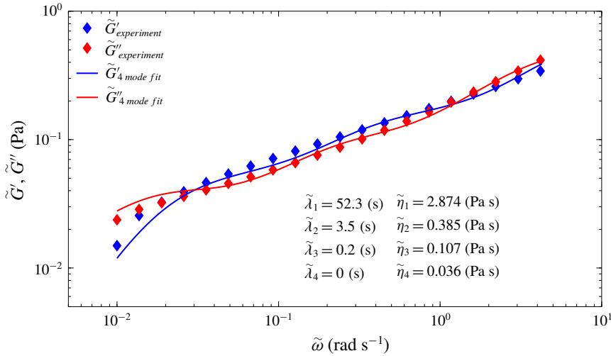
FIGURE 6. (Colour online) Variation of the storage and loss modulus versus the frequency for the solution of 190 ppm PAA in 70:30 glycerine–water at \tilde{T} = 20 (°C).
