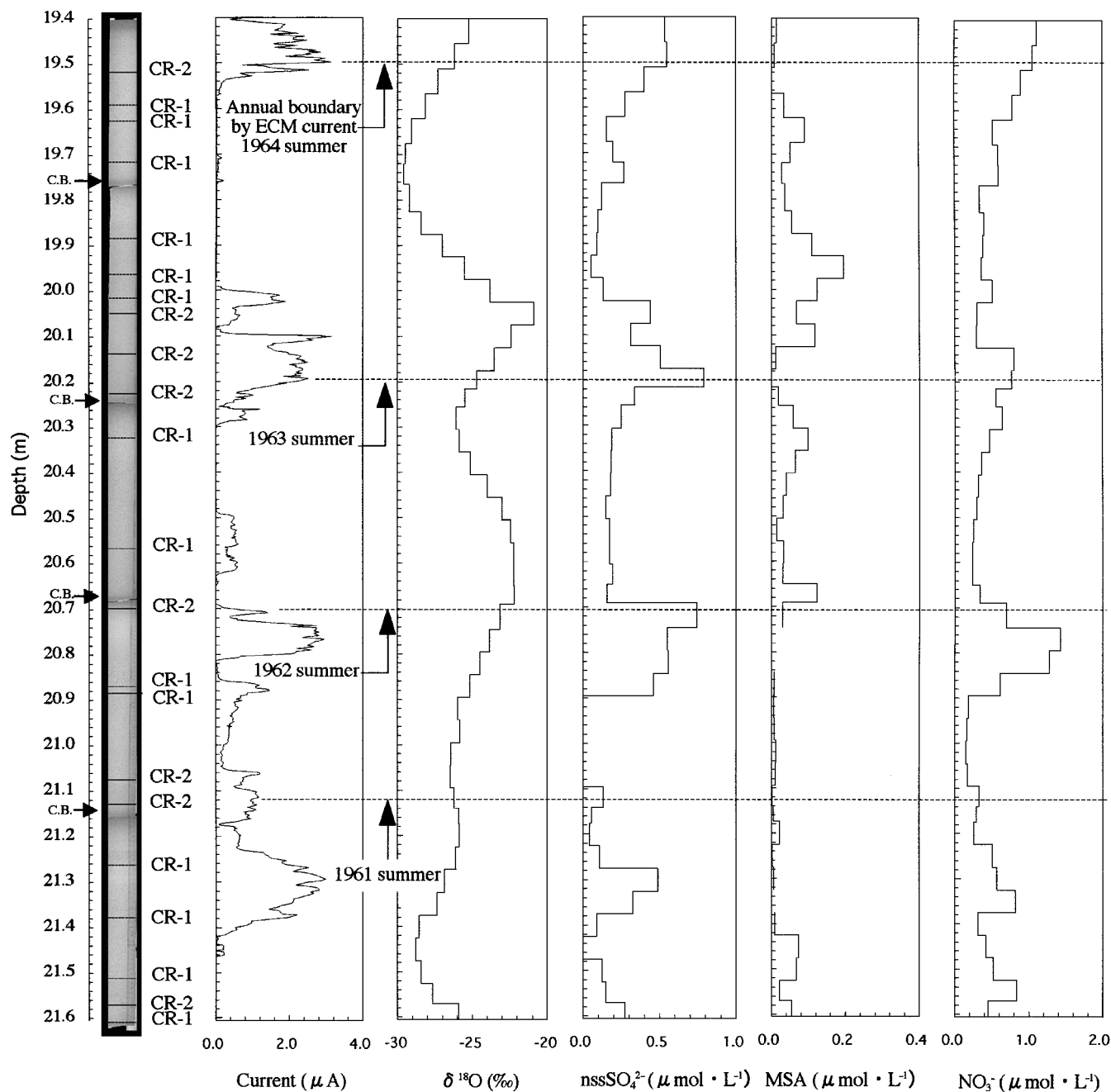
Fig. 4. Profiles of visual stratigraphy, ECM current, \delta^{18}\text{O} , \text{nssSO}_4^{2-} , MSA and \text{NO}_3^- from 19.40 to 21.60 m. Visual stratigraphy is composed of mosaicked pictures continuously taken by digital video camera along the ice core. Ice crust CR-1 is multi-layered and includes air bubbles. Ice crust CR-2 is identified as probably summer layers at depths of 19.45–19.50, 20.17–20.21 m, 20.74–20.79 and 21.09–21.14 m. C.B. signifies a break in the core.
