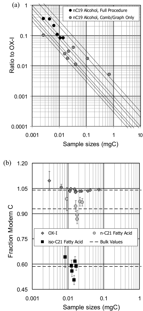
Figure 4 (a) Indirect MC contamination assessment for the full CSRA procedure (black symbols) and combustion + graphitization steps only (gray symbols) using n\text{C}_{19} alcohol standard ( \Delta^{14}\text{C} = -999\text{‰} ). Diagonal lines represent fixed amounts of MC contamination from 0.2 to 3 \mu\text{g C} (left to right); (b) Indirect DC contamination assessment for the full CSRA procedure ( n\text{C}_{21} fatty acids, light gray circles) and combustion + graphitization steps only (OX-I, dark gray diamonds). Measured values for a standard of intermediate radiocarbon composition ( iso\text{C}_{21} fatty acids, black squares) are also shown. Horizontal dashed lines denote the corresponding consensus values based on bulk-level measurements. All data were corrected for machine-induced isotopic fractionation.
