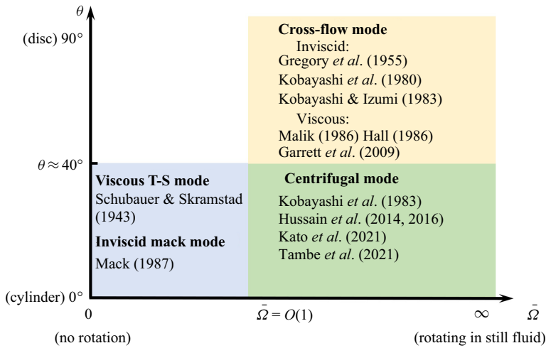
Figure 2. Sketch of the instability modes in the \theta - \bar{\Omega} space.
