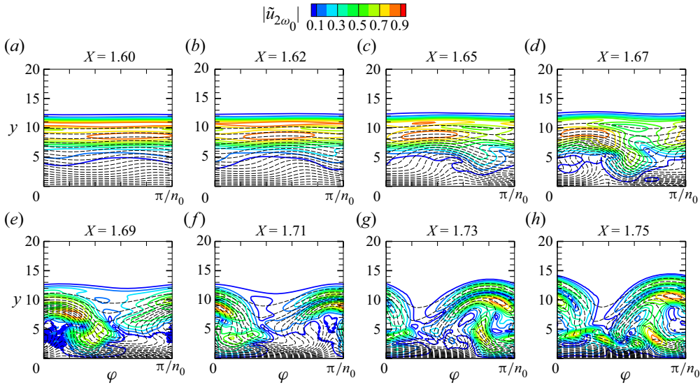
Figure 20. Contours of the perturbation profiles |\tilde{u}_{2\omega_0}| in the y - \varphi plane for case VI. The dashed lines denote the contours of \tilde{\Phi}_B(y, \varphi) .
