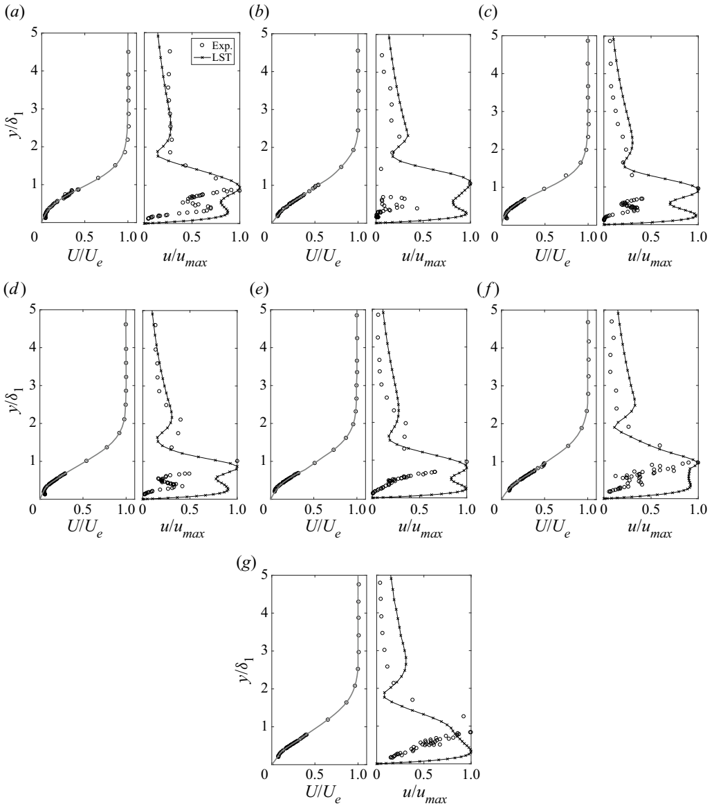
Figure 18. Experimental filtered disturbance profiles in the wall-normal direction compared with the eigenfunction for the most amplified frequency from LST. Experimental streamwise disturbance profiles are computed by applying a bandpass filter corresponding to the lost amplified frequency band from the PSD. (a) Natural case; [110–150 Hz] at x = 0.425c , (b) Tu = 0.64\% , \Lambda_u = 4.6 mm [160–200 Hz] at x = 0.400c , (c) Tu = 1.21\% , \Lambda_u = 8.7 mm [180–220 Hz] at x = 0.425c , (d) Tu = 1.23\% , \Lambda_u = 10.3 mm [180–220 Hz] at x = 0.400c , (e) Tu = 1.31\% , \Lambda_u = 8.3 mm [180–220 Hz] at x = 0.400c , (f) Tu = 1.63\% , \Lambda_u = 12.3 mm [180–220 Hz] at x = 0.450c and (g) Tu = 2.97\% , \Lambda_u = 15.4 mm [255–295 Hz] at x = 0.425c .
