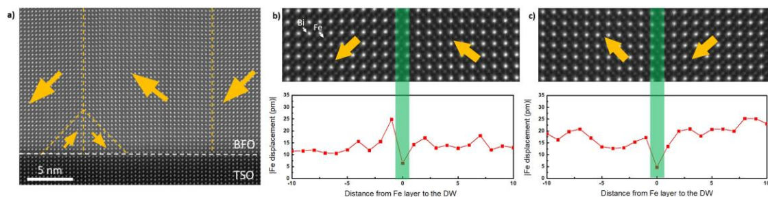
Figure 2. 109^\circ DWs and displacement measurements (a) Cross-sectional HAADF STEM image. (b) & (c) Fe in-plane displacement measurements in the regions labeled as b and c in (a), respectively.
