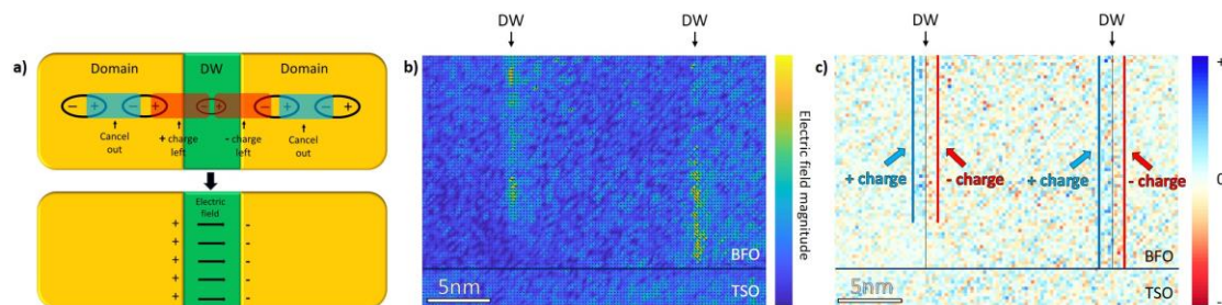
Figure 1. 109^\circ DW model and low-convergence angle 4D STEM results. (a) Schematic of a 109^\circ DW with displacement discontinuity. (b) Electric field and (c) charge density mappings are collected by using low-convergence angle 4D STEM.
