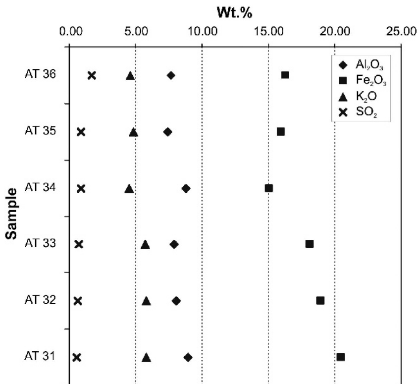
Figure 3. Chemical variations of glauconite grains in surface Layer 16; mean Al 2 O 3 , Fe 2 O 3 , K 2 O, and SO 2 contents (mean of 14 analyses per sample) of glauconite grains from samples AT31 (base) to sample AT36 (top of Layer 16).
