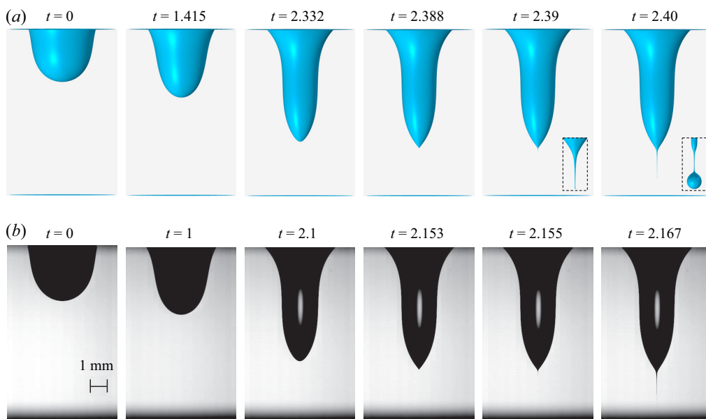
Figure 2. Side-view snapshots of an electrified pendant droplet during the tip streaming process at different dimensionless times for \theta_0 = 105.6^\circ , Oh = 0.0431 , Ca_E = 0.11 , Bo = 1.27 and \alpha = 157.5 . Here the electric field is created by two parallel electrodes. The insets in the last two images show the magnified view of the jet's tip. Reprinted with permission from Ferrera et al. (2013). Copyright 2013 AIP Publishing.
