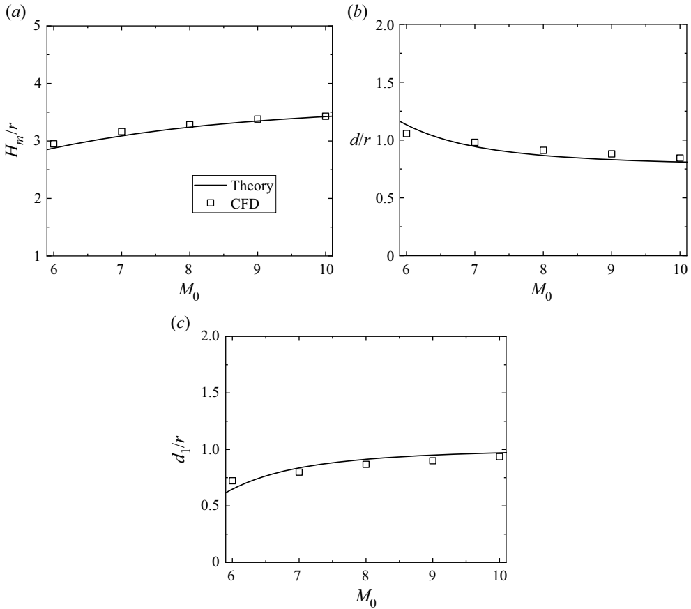
Figure 18. Normalized theoretical results and numerical simulations for free stream Mach number M_0 ranging from 6 to 10 at R/r = 3 and \beta = 24^\circ : (a) the MS height H_m ; (b) the triple point position d ; and (c) the relative position d_1 of the triple point T and the elbow.
