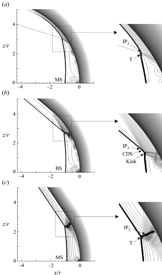
Figure 21. Variations of shock interaction configurations with half-span angle \beta at M_0 = 6 and R/r = 5.5 : (a) the primary MR, \beta = 16^\circ ; (b) sRR, \beta = 40^\circ ; and (c) the primary MR, \beta = 56^\circ .
