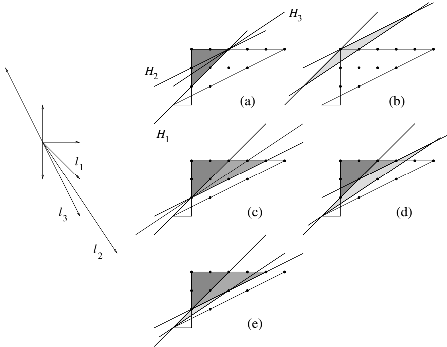
FIGURE 3. The fan of \mathbb{F}_2 blown up three times and the hyperplane arrangements corresponding to the divisors (a) 3Q - P - 2R_1 , (b) 3Q - P - 2R_3 , (c) 3Q - P - 2R_1 - 2R_2 , (d) 3Q - P - 2R_1 - R_2 - 2R_3 , (e) 3Q - P - 2R_1 - 2R_2 - R_3 .
