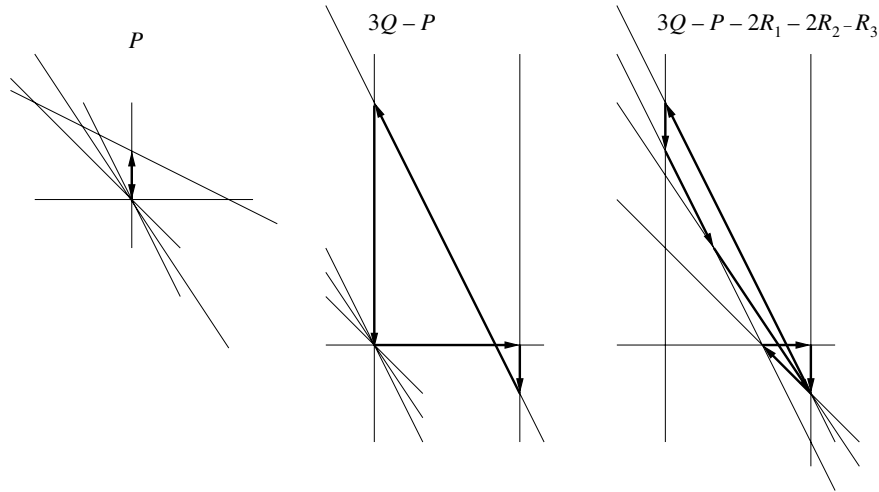
FIGURE 4. The fan of Figure 3 and the polygonal lines associated to the divisors P , 3Q - P , and 3Q - P - 2R_1 - 2R_2 - R_3 . The picture shows the hyperplane arrangements associated to these divisors rotated by 90 degrees and the polygonal lines embedded into them.
