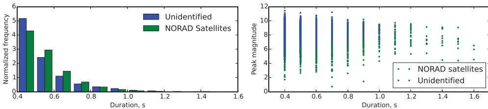
Figure 2. Comparison of durations (left panel) and brightness (right panel) of rapid flashes detected by Mini-MegaTORTORA and identified/non-identified with NORAD satellites.
