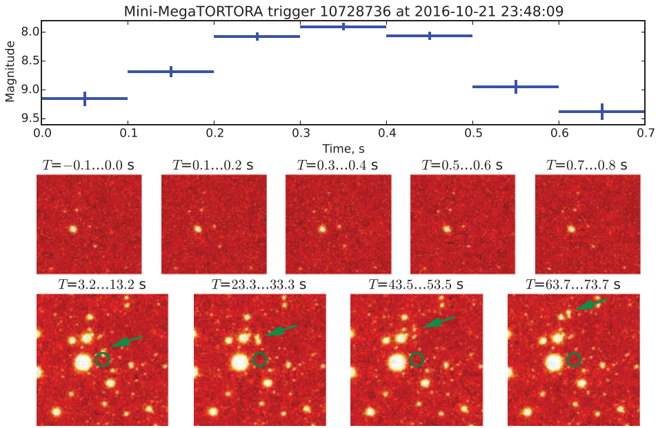
Figure 1. Example of a rapid optical flash independently detected and followed-up by Mini-MegaTORTORA and not identified with satellites from NORAD database. Upper panel – light curve with 0.1 s temporal resolution, middle panel – corresponding detection images (50' x 50' around the event), lower panel – follow-up images with 10 s exposures that clearly reveal the satellite, marked by arrow, slowly moving away from the flash position, marked by circle.
