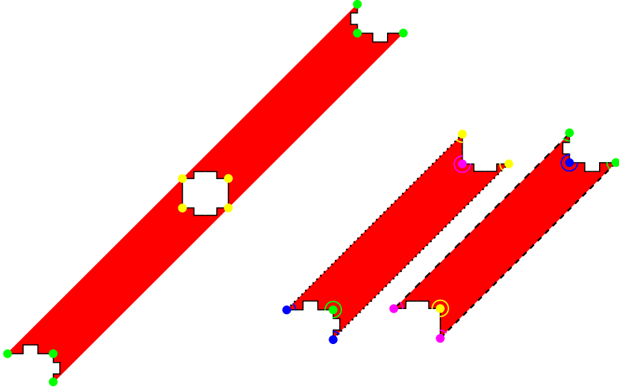
FIGURE 12. The subset R \setminus \partial R of M(E_1) and its completion \bar{R}(E_1) in the case of two intersection points.
