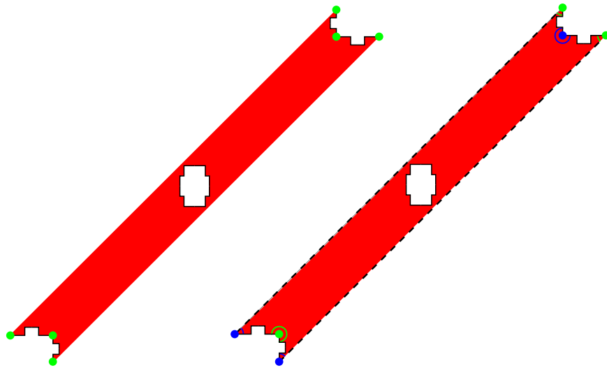
FIGURE 10. The subset R \setminus \partial R of M(E_1) and its completion \bar{R}(E_1) .
