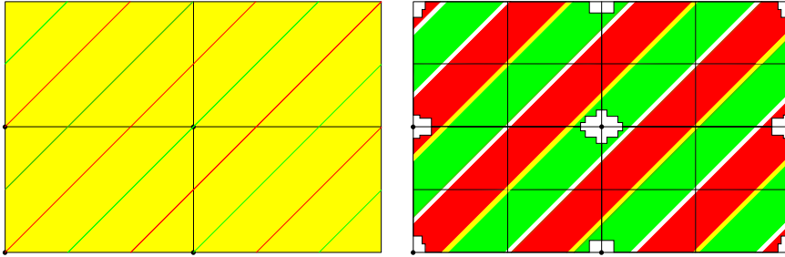
FIGURE 9. Two periodic orbits ( red and green ) on \mathbb{T}_{m,n} and the corresponding cylinders on M(E_1) .
