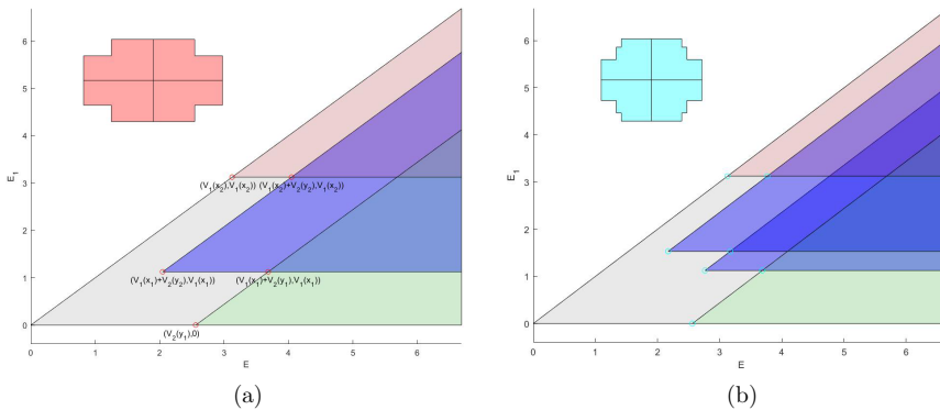
FIGURE 5. Impact energy-momentum bifurcation diagram: (a) for a symmetric cross (one concave corner with multiplicity4); (b) symmetric two-step cross (two concave corners each with multiplicity4). Here, due to symmetry, each blue wedge corresponds to four overlapping wedges, so R^{(E, E_1)} \cap P includes 4k concave corners if and only if (E, E_1) is in a region covered by 4k overlapping shaded blue regions. Only for these regions is the level sets genus greater than 1. The pink (respectively, light-green) regions correspond to level sets that impact the extreme vertical (respectively, horizontal) sides.
