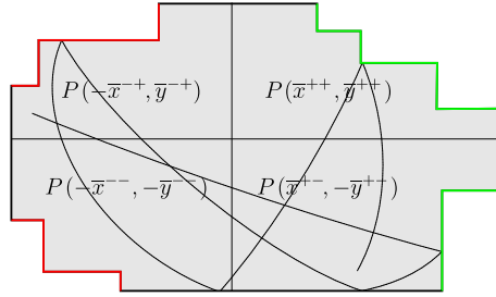
FIGURE 1. The living space of the particle.
