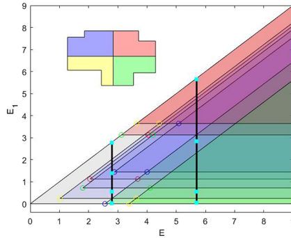
FIGURE 6. Impact energy-momentum bifurcation diagram for the asymmetric cross shown in Figure 4 (four distinct concave corners). The colored circles correspond to the energies of the corners of the corresponding colored staircase polygons shown in the inset. All corners have distinct partial energies, so R^{(E, E_1)} \cap P includes k concave corners if and only if (E, E_1) is in a region covered by k overlapping blue regions. Only for these regions is the level sets genus greater than 1. The pink (respectively, light green) regions include extremal vertical (respectively, horizontal) boundaries. The two vertical lines indicate the energies E = 2.7, 5.7 and the cyan squares on these lines correspond to the E_1 values of the rectangles shown in Figure 4.
