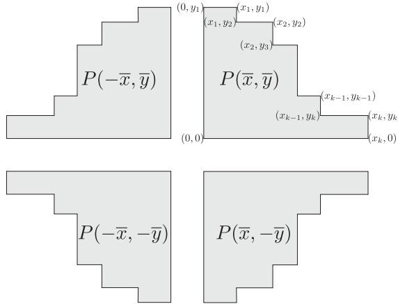
FIGURE 2. Staircase polygons P(\bar{x}, \bar{y}) , P(-\bar{x}, \bar{y}) , P(\bar{x}, -\bar{y}) , P(-\bar{x}, -\bar{y}) .
