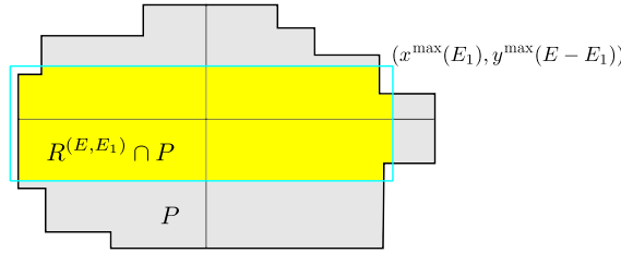
FIGURE 3. A projected rectangle and the staircase polygon. Cyan—the projected rectangle. Yellow—the polygon R^{(E, E_1)} \cap P includes three concave corners, thus, by Theorem 1.2, g(E, E_1) = 4 .
