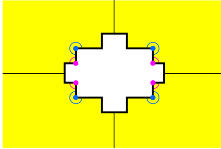
FIGURE 8. Singularities of M(E_1) .
