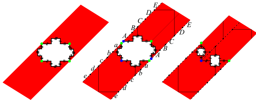
FIGURE 11. This figure shows the construction of \bar{R}(E_1) around removed polygons. In particular, it indicates the rules for gluing segments with the same labeling. The rightmost part of the figure shows the resulting surface after gluing the segments labeled with capital letters.
