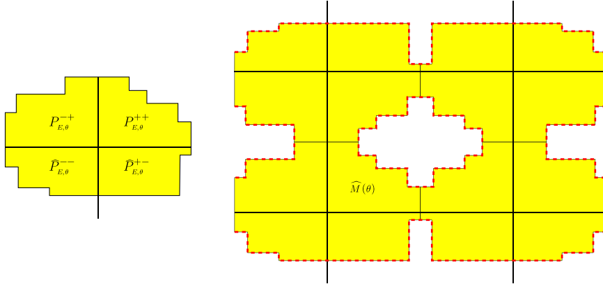
FIGURE 15. The extended billiard table \widehat{P}_{E,E_1} and \widehat{M}(E_1) .
