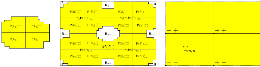
FIGURE 7. The billiard table \mathbf{P}(E_1) , the translation surface M(E_1) and the marked torus \mathbb{T}_{m,n} .
