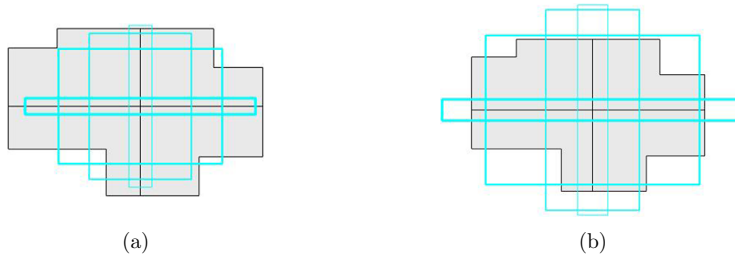
FIGURE 4. The intersection of a star-shaped polygon (gray) with four iso-energy projected rectangles (cyan) at (a) E = 2.7 and (b) E = 5.7 energy values. By Theorem 1.2, the genera of the corresponding iso-energy level sets for the four R^{(E, E_1)} rectangles shown are, for increasing E_1 (a) g(E = 2.7, E_1) = \{1, 2, 4, 1\} (b) g(E = 5.7, E_1) = \{1, 2, 5 = g_{\max}, 1\} . The potentials here are quadratic with \omega_1 = 1, \omega_2 = 0.8\sqrt{2} .
