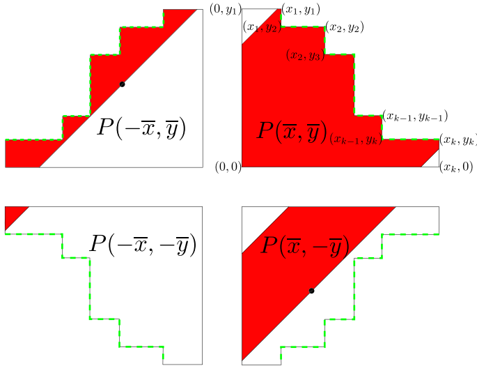
FIGURE 13. New basic polygons.
