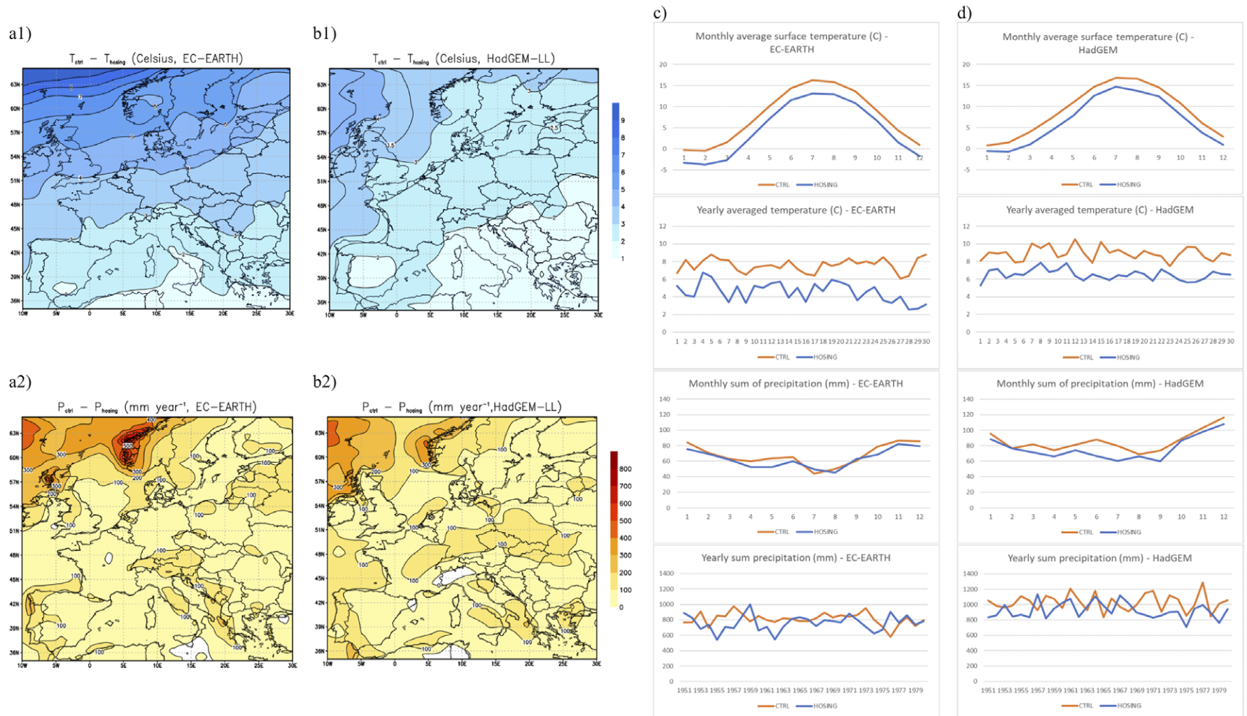
Figure 3. Difference in temperature (°C, upper panels) and precipitation (mm year -1 , lower panels) between the control simulation and hosing experiment for EC- Earth3 (a) and HadGEM-LL (b). Monthly and yearly mean temperatures and monthly mean precipitation for the EC-Earth3 (c) and HadGEM3 (d) model results from Bellomo et al. (2023) and Jackson et al. (2023), for control and hosing experiments. This a spatial average for an area bounded by 48°N and 54°N and 3°E and 8°E.
