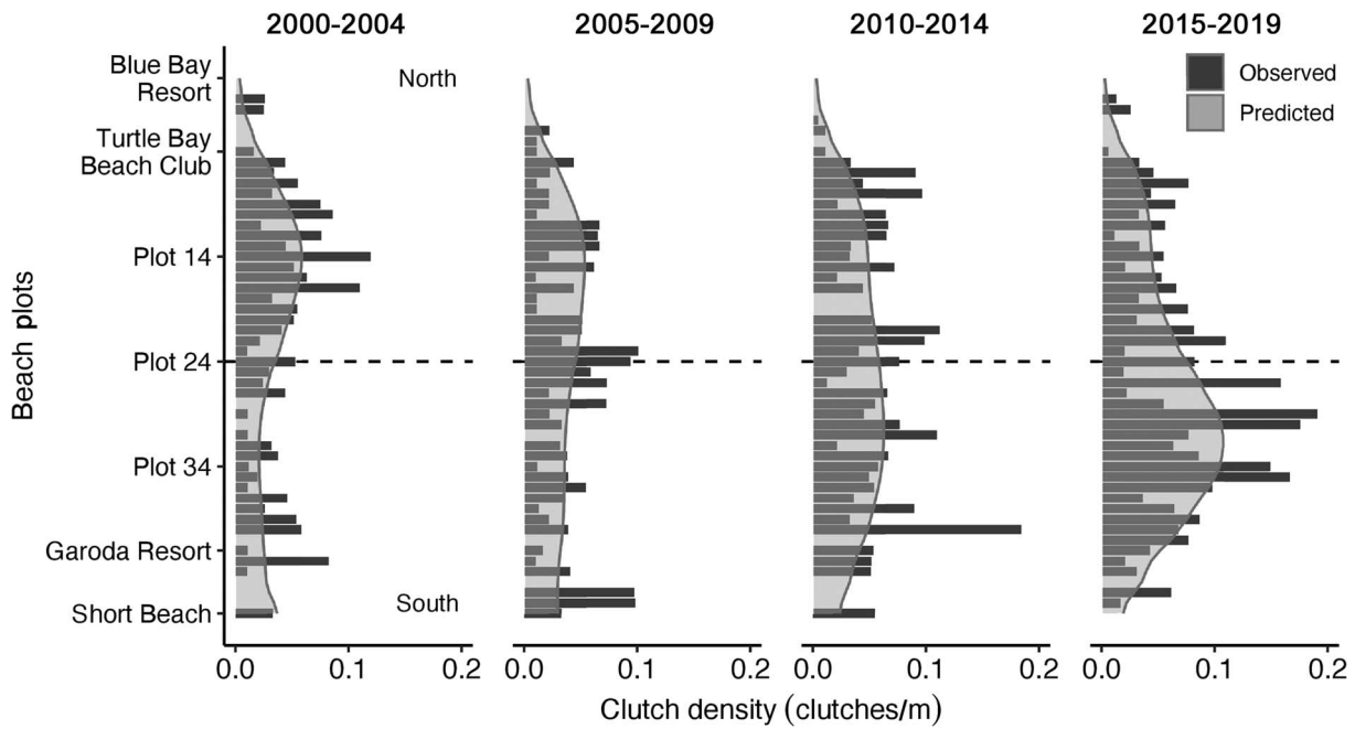
FIG. 6 Observed and predicted distribution of clutches for all four turtle species combined ( n = 855 ) laid in Watamu Marine National Park, Kenya. Clutch density per beach plot from north to south during four five-season bins. The dashed line indicates the division between the northern and southern halves of Watamu Marine National Park. Locations from Fig. 1d are indicated here for reference.
