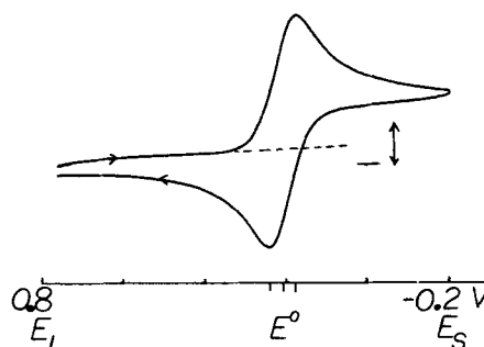
Figure 3. Cyclic voltammetric experiment for the reduction of \text{Fe}(\text{CN})_6^{3-} (4 mM) at a bare Pt electrode in 0.7 M NaCl. In the forward potential sweep past E^\circ (from E_i to E_s ) a reduction peak is observed. In the reverse potential sweep past E^\circ (from E_s to E_i ) an oxidation peak is observed. The bar defines 0.1 \mu\text{A} of current. The peak height, measured from the extrapolated baseline, is dependent on scan rate, diffusion coefficient, and concentration of the complex. The formal potential for the reduction is determined from the midpoint between the two current peaks.
