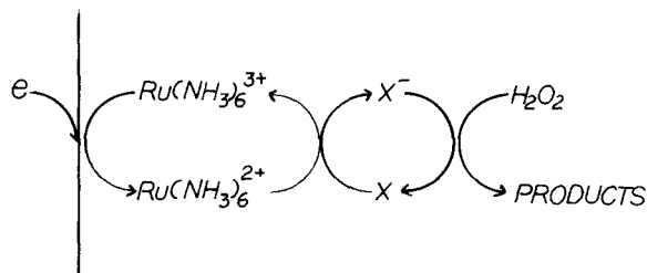
Figure 7. A charge shuttle. Ru(NH_3)_6^{3+} , carries an electron from electrode surface to a fixed electroactive site within the clay, X, which catalyzes the reduction of H_2O_2 . Reaction mechanism proposed by Oyama and Anson (1986).
