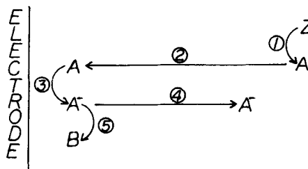
Figure 2. Possible rate-limiting steps in an electrochemical reaction. (1) An electroinactive species, Z , converts to A . (2) A diffuses to the electrode surface. (3) A is reduced (or oxidized) to its product A^- . (4) A^- diffuses away from the electrode surface. (5) A^- is converted to another chemical species, B .
