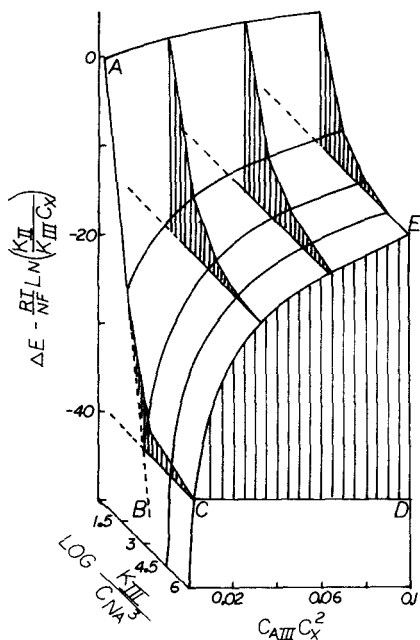
Figure 4. Plot of difference between apparent formal potential for the reduction of A^{3+} within the clay film and formal potential at a bare electrode ( \Delta E ) as a function of the divalent and trivalent exchange constants, K_{II} and K_{III} , the total number of exchange sites present, C_x , and the bathing solution concentrations of A^{3+} , C_{AIII} , and Na^+ , C_{Na} . \Delta E is offset by a constant related to the exchange constants and C_x . In all cases, potential shifts positive with bathing solution concentration of A^{3+} , C_{AIII} . The 59 mV/decade change in potential with [Na^+] (line AB) was predicted by Naegeli et al. (1986).
