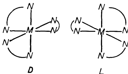
Figure 6. Spatially unique trisdiimine metal complexes (enantiomers) of the form ML_3 in which L is a ligand containing two N groups, such as phenanthroline or bipyridine. D is the mirror image of L. The two enantiomers can be resolved by their optical polarization.
