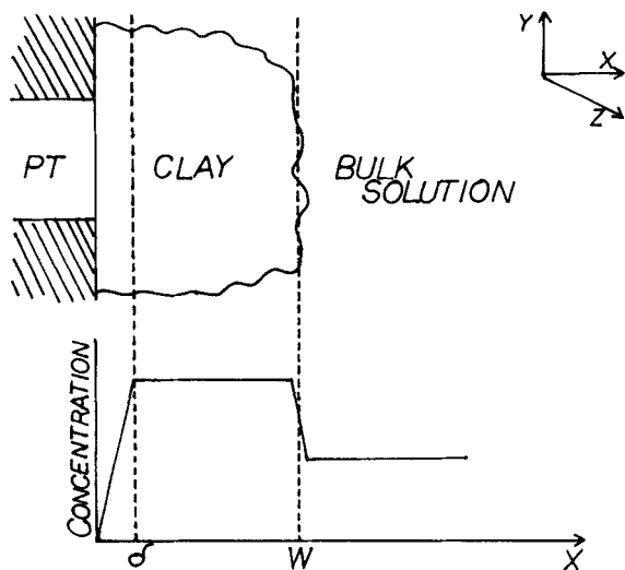
Figure 1. Diagram of a clay-modified electrode. Underlying Pt electrode is encased in an insulating material (cross hatched area) and covered with clay. Concentration of cationic species in solution ( x \rightarrow \infty ) is enhanced within the clay film ( x < w ) due to the negative charge of the clay and is depleted within the diffusion layer ( x < d ) at the surface of the electrode via a reduction/oxidation reaction at the electrode. Diffusion occurs primarily perpendicular to electrode surface in the x direction compared with y and z directions parallel to the electrode surface.
