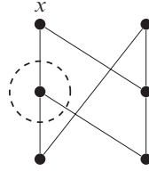
FIGURE 2. A model on the variables X = \{x\} , where the marked subset is the domain on which the implication \neg \rightarrow x \rightarrow x is not valid.
