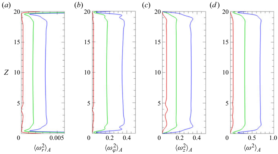
Figure 7. Profiles of the (r, \phi) -averaged enstrophy ( \langle \omega^2 \rangle_A ) and the components ( \langle \omega_i^2 \rangle_A ) for three values of V_E (red, V_E = 500 ; green, V_E = 600 ; blue, V_E = 700 ). Here, \langle X \rangle_A denotes an area average over the annulus section at a given z , \langle X \rangle_A = (1/A) \iint X \, dA , where dA = r \, dr \, d\phi .
