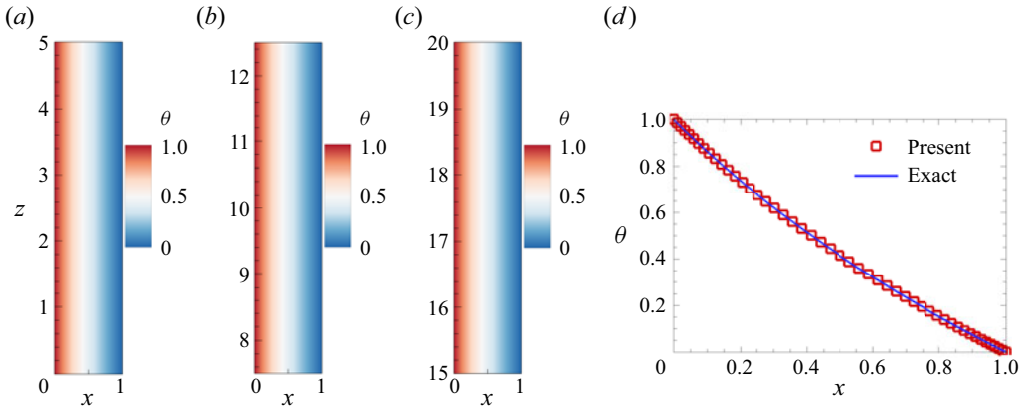
Figure 2. The temperature fields for V_E = 450 ; contours of temperature (a) near the bottom plate, (b) in the middle, (c) near the top plate and (d) the profile of temperate along the radial direction at the midplane z = 10 . The symbols are plotted for every other obtained point for clarity.
