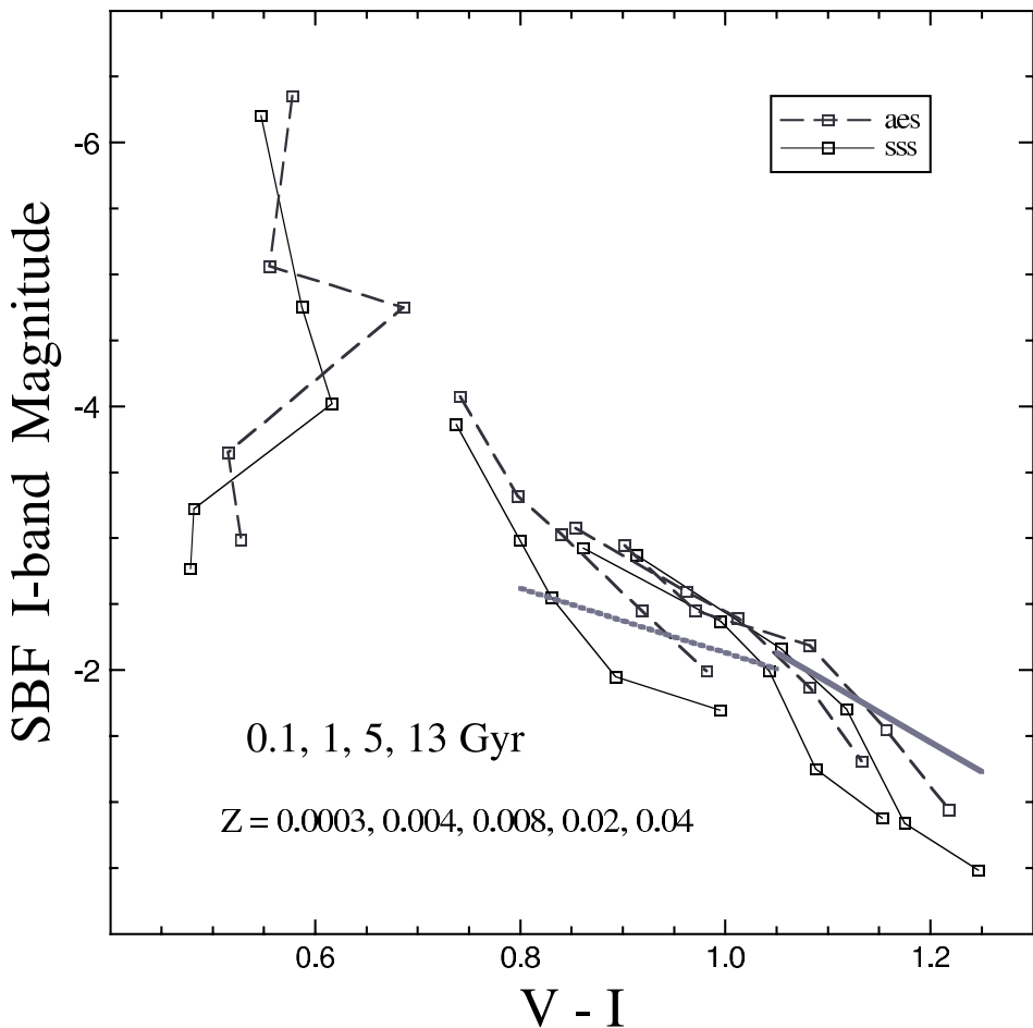
Figure 1. V - I vs. SBF I-band Magnitude at 0.1, 1, 5, and 13 Gyr (left to right). Solid lines with squares are solar-scaled models while dashed lines with squares are alpha-enhanced models. At given ages, SBF I-band Magnitudes become fainter and V - I colors become redder, in general, with increasing metallicity. Two observational fiducial lines are compared with our theoretical models (see text).
