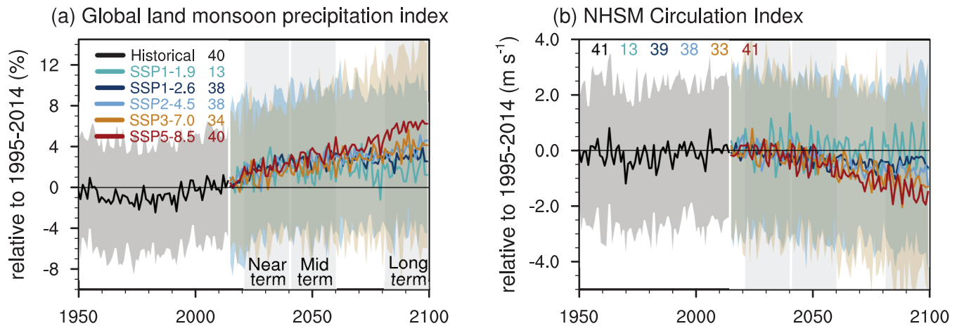
Figure 4.14 | Time series of global land monsoon precipitation and Northern Hemisphere summer monsoon (NHSM) circulation index anomalies. (a) Global land monsoon precipitation index anomalies (unit: %) defined as the area-weighted mean precipitation rate in the global land monsoon domain (as defined by Wang et al. (2013a) for the CMIP6 historical simulation (1950–2014) and five SSPs (2015–2100). (b) Anomalies in NHSM circulation index (unit: \text{m s}^{-1} ), defined as the vertical shear of zonal winds between 850 and 200 hPa averaged in a zone stretching from Mexico eastward to the Philippines ( 0^{\circ} – 20^{\circ}\text{N} , 120^{\circ}\text{W} – 120^{\circ}\text{E} ; Wang et al., 2013a) for the CMIP6 historical simulation and five SSPs. One realization is averaged from each model. Anomalies are shown relative to the present-day (1995–2014) mean. The curves show averages over the simulations, the shadings around the SSP1-2.6 and SSP3-7.0 curves show 5–95% ranges, and the numbers near the top show the number of model simulations used. Further details on data sources and processing are available in the chapter data table (Table 4.SM.1).
