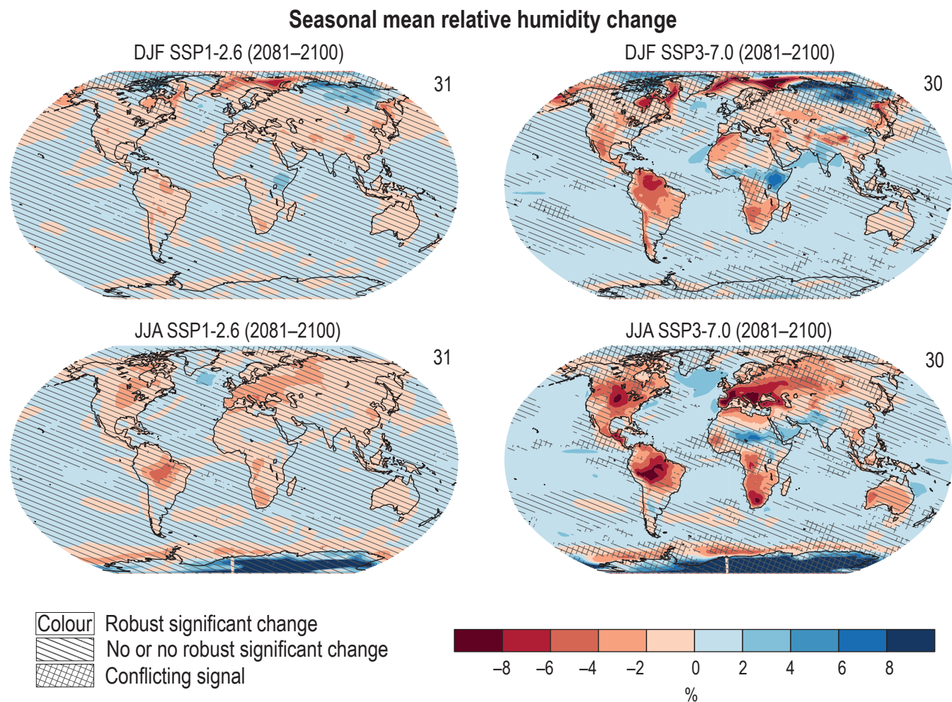
Figure 4.23 | Long-term changes in seasonal mean relative humidity. Displayed are projected spatial patterns of multi-model mean change (%) in seasonal ( top ) December–January–February (DJF) and ( bottom ) June–July–August (JJA) mean near-surface relative humidity in 2081–2100 relative to 1995–2014, for (left) SSP1-2.6 and (right) SSP3-7.0. The number of models used is indicated in the top right of the maps. No overlay indicates regions where the change is robust and likely emerges from internal variability, that is, where at least 66% of the models show a change greater than the internal variability threshold (Section 4.2.6) and at least 80% of the models agree on the sign of change. Diagonal lines indicate regions with no change or no robust significant change, where fewer than 66% of the models show change greater than the internal-variability threshold. Crossed lines indicate areas of conflicting signals where at least 66% of the models show change greater than the internal-variability threshold but fewer than 80% of all models agree on the sign of change. Further details on data sources and processing are available in the chapter data table (Table 4.SM.1).
