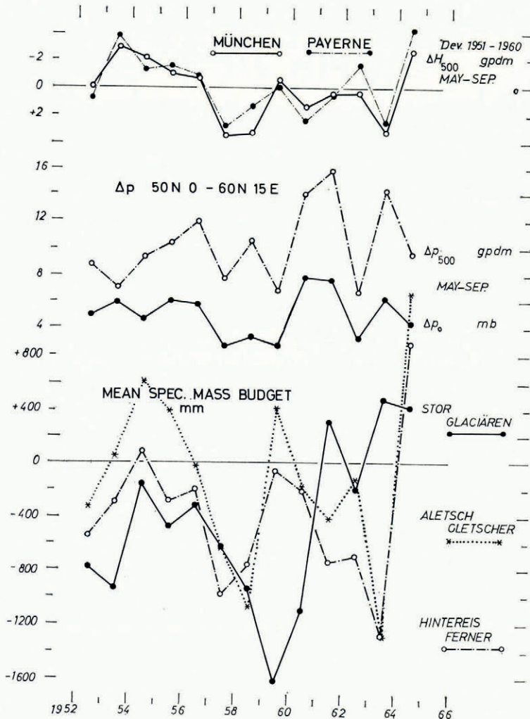
Fig. 4. Mean specific mass budget in mm of water of Grosser Aletschgletscher, Hintereisferner and Storglaciären 1952/53 to 1964/65. Mean pressure difference (surface and 500 mbar) between lat. 50° N., long. 0° E. and lat. 60° N., 15° E. (European north-westerlies), May to September 1953 to 1965. Mean deviation from the 1951-1960 average height of the 500 mbar surface over München and Payerne, May to September 1953 to 1965 in geopotential decametres (gpdm)
