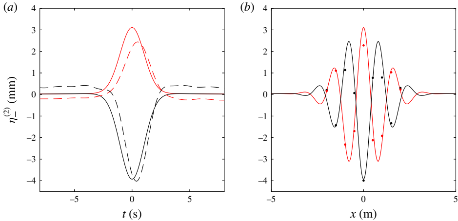
FIGURE 15. (Colour online) Temporal (a) and spatial (b) evolution of the wave-averaged surface elevation \eta_{-}^{(2)} at the focus point ( x = 0, y = 0 ) for two wave groups colliding head-on ( \Delta\theta = 180^\circ ). The red lines correspond to two groups that are in phase ( \mu_1 = \mu_2 ) and the black lines to groups that are out of phase ( \mu_1 - \mu_2 = 180^\circ ). The multiple-scale solution (2.15) is given by the continuous lines, and the measurements by the dashed lines in (a) and the dots in (b).
