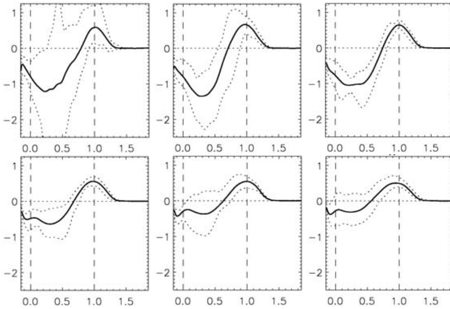
Figure 2. Results for rapid rotation ( Co = 10 ). \alpha_{yy} = \alpha_{\phi\phi} averaged over time in dimensionless units as a function of depth z in the simulation box. Dimensionless units are the same as in Fig. 1. From top left to bottom right the graphs represent simulations between 105 and 180 degrees (= south pole) of colatitude, at 15 degree intervals. Notice the rotational quenching of \alpha_{\phi\phi} in the unstable region at high latitudes, and the region where \alpha_{\phi\phi} has the opposite sign near z = 1 , the base of the unstable layer.
