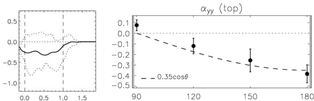
Figure 1. \alpha_{yy} = \alpha_{\phi\phi} for slow rotation ( Co = 1 ). Left: time average in dimensionless units as a function of depth z in the simulation box. The dimensionless unit of \alpha_{yy} is 0.01\sqrt{dg} , that of depth is d , the thickness of the unstable region; g is the gravity acceleration. The simulation box represents a colatitude of 150 degrees ( 90 = \text{equator} , 180 = \text{south pole} ). Right: time average in dimensionless units evaluated at z = 0 (in the unstable layer) as a function of colatitude. The dashed curve is a \cos fit. In the overshoot layer \alpha_{\phi\phi} vanishes.
