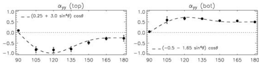
Figure 3. \alpha_{yy} = \alpha_{\phi\phi} in the rapid rotation regime ( Co = 10 ), averaged over time evaluated at two different depths in dimensionless units as a function of colatitude (90 = equator, 180 = south pole). The dashed curve is a spline fit. Left: z = 0 (unstable region). Right: z = 1 (stable layer).
