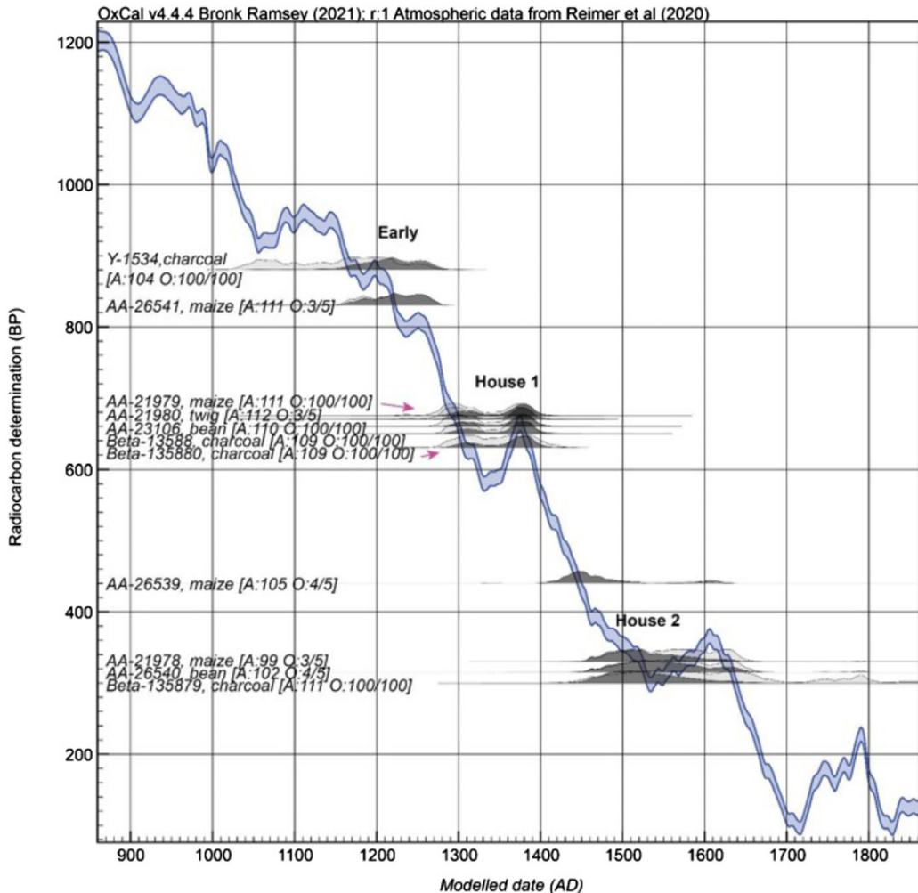
Figure 8 Modeled (dark gray) and non-modeled (light gray) probability distributions (posterior densities) for Roundtop (model with no additional constraints) shown placed against the IntCal20 radiocarbon calibration curve. The three distinct periods of human activity are indicated. AA-26539 may indicate another occupation phase or might be associated with the overall period of House 2 activity at the site.
