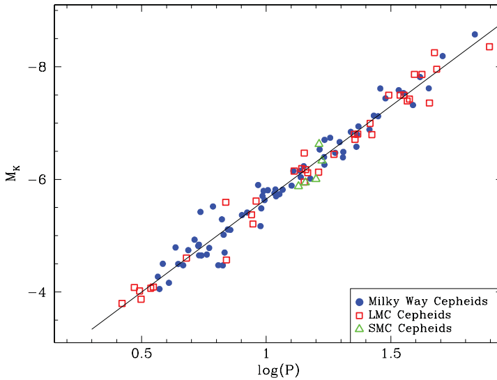
Figure 2. Composite K -band Cepheid PL relation obtained from IRSB distances to 70 Cepheids in the MW, 36 in the LMC, and five in the Small Magellanic Cloud (SMC). The K -band PL relation is independent of metallicity in the range from solar to the typical SMC Cepheid metallicity.
