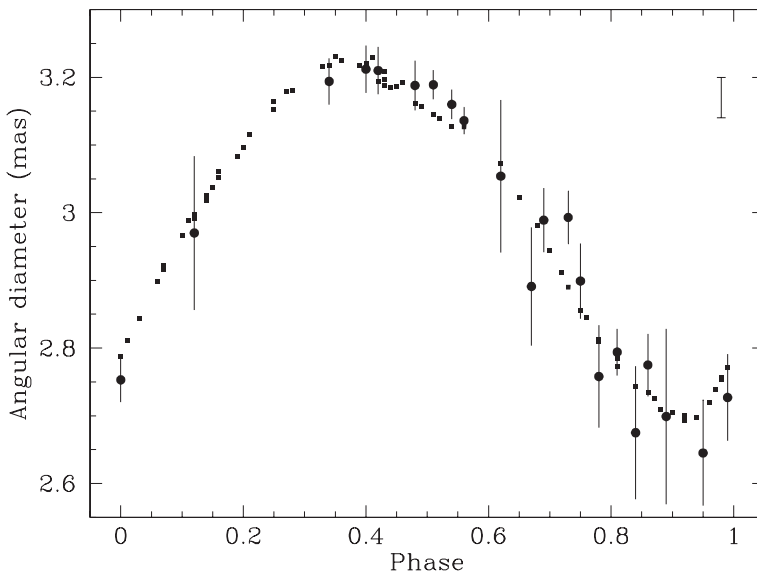
Figure 1. Black bullets: Interferometric angular-diameter measurements for the Cepheid \ell Car. Blue squares: Angular diameters calculated using the IRSB technique. The agreement is at the 1% level (see Kervella et al. 2004b).
