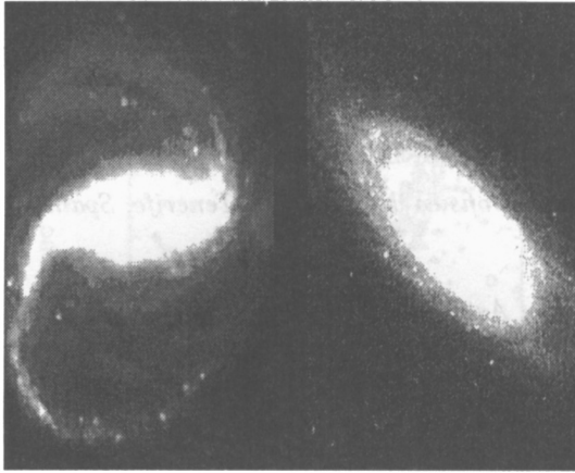
Figure 1. I band images of NGC 7479 (left) and NGC 7606 (right).
