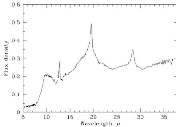
Figure 2. Spitzer mid-IR spectrum of the Li-rich K giant star PDS 68 between 5 and 38 \mu\text{m} presenting the UIE features superposed on a strong continuum emission (de la Reza et al. 2015). The spectrum was taken from the Cornell Atlas of Spitzer /IRS sources (CASSIS, Leboutteiller et al. 2011).
