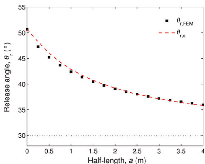
Fig. 7. Evolution of the release angle, \theta_r , as a function of the half-length, a , of the weak spot. Black squares: finite-element results. Red dashed curve: theoretical stress rupture threshold.
