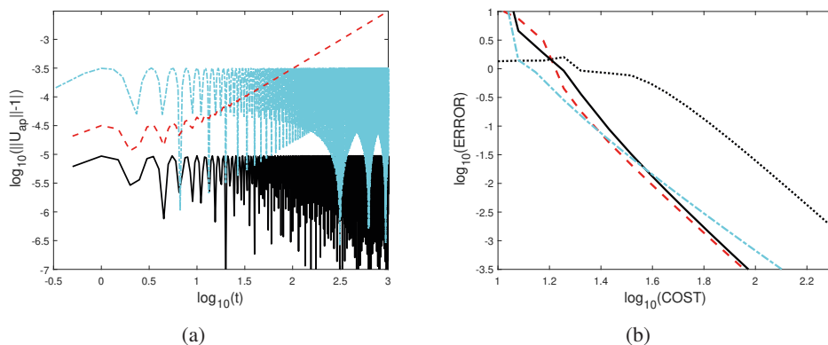
Figure 7.1. (a) Evolution of error in unitarity for system (7.13) integrated with third- and fourth-order splitting methods with complex coefficients. (b) Efficiency diagram computed for a final time t_f = 10 . Different patterns in the coefficients lead to different qualitative behaviour.
