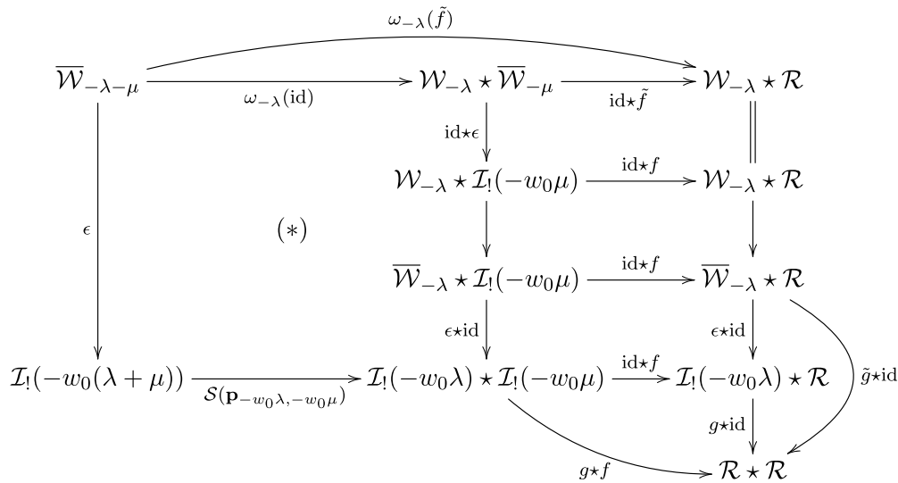
FIGURE 3. Comparing ring structures in Theorem 6.2.
