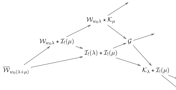
FIGURE 2. Octahedral diagram for Lemma 5.16.
