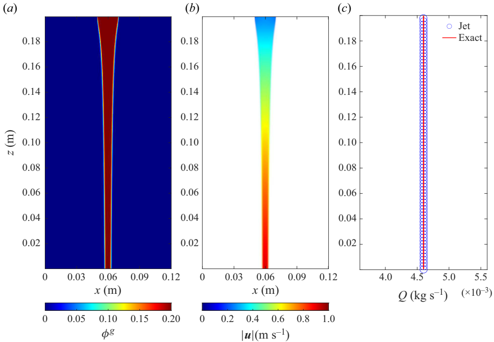
Figure 11. Numerical simulation of a free-falling jet using the the partially regularized \mu(I) -rheology in the absence of wall friction and interface-sharpener forces. (a) The volume fraction of granular material in the free-falling jet, and (b) the velocity magnitude. (c) The blue circles represent the computed width-averaged flow rate through the jet at each z coordinate, while the red line represents the flow rate input by the boundary conditions, i.e. Q = 0.0046 \text{ kg s}^{-1} .
