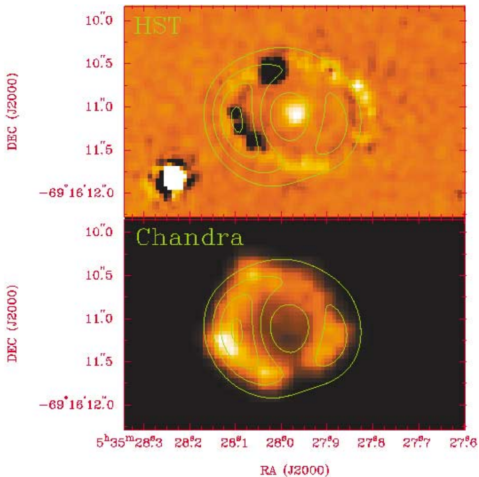
Figure 10 Multi-wavelength comparisons of SNR 1987A. The upper panel overlays HST and ATCA observations of SNR 1987A: the false-colour image represents the difference of HST WFPC2 images in the F6565N filter, obtained by subtracting an image taken in 1998 February from a similar image taken in 1999 April (Lawrence et al. 2000), while the contours correspond to the super-resolved 2000.8-epoch ATCA image, using contour levels of 1.1, 2.2, 3.3, and 4.4 mJy beam -1 . The lower panel overlays Chandra and ATCA observations — the false-colour represents a super-resolved Chandra ACIS-S image covering the energy range 0.3–8 keV at epoch 1999.8 (Burrows et al. 2000), while the contours indicate radio data as in the upper panel.
