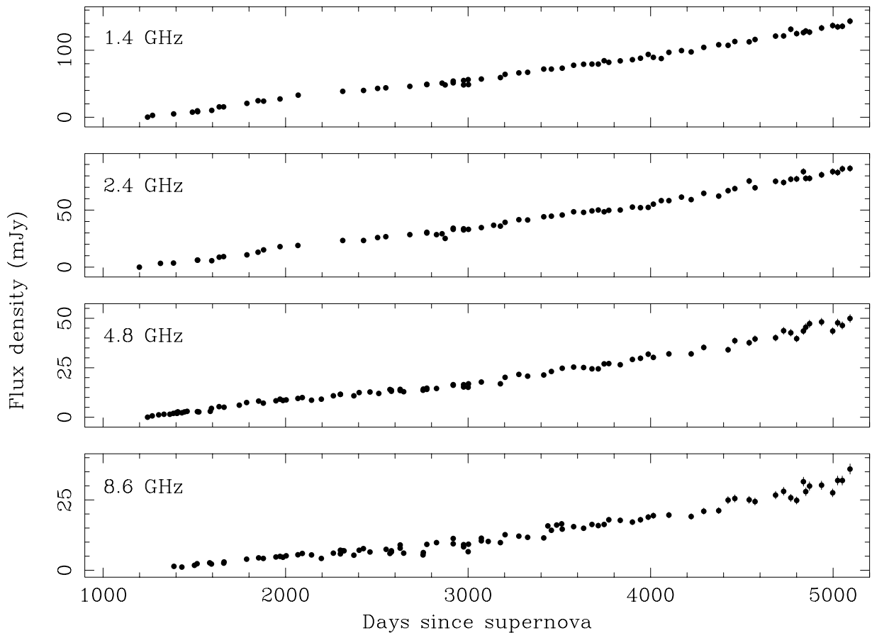
Figure 1 Flux densities of SNR 1987A from 1990 August to 2001 February observed with the Australia Telescope Compact Array.
