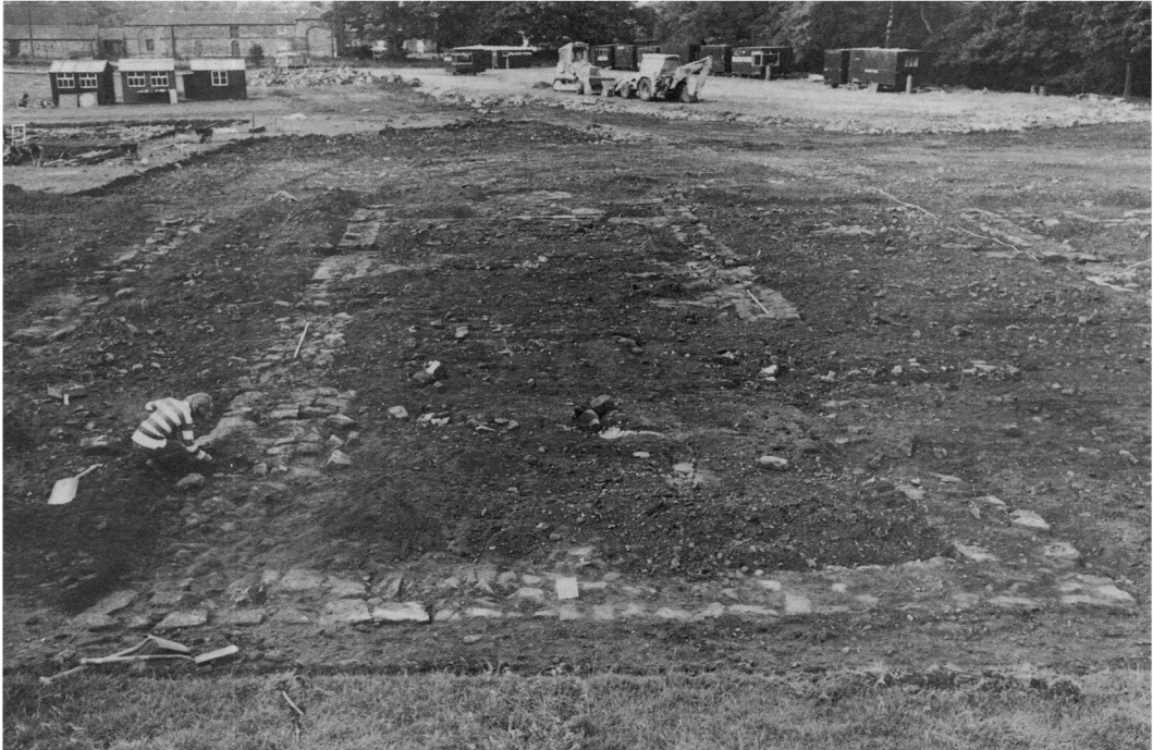
A. Greta Bridge. East vicus . Building F. View south (scale 2 m). (p. 122)
