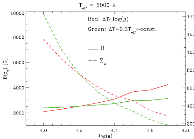
Figure 1. Variation of field strength B (solid lines) and the Wilson depression Z_w (dashed lines) against \log(g) for T_{eff} = 6000K
