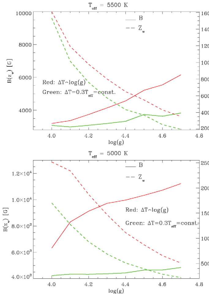
Figure 2. Same as Fig. 1 but for T_{eff} = 5500K (top) and 5000K (bottom)
