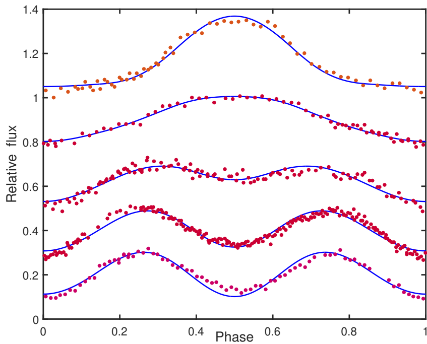
Figure 8: Theoretical (lines) and observed (dots) light curves of WISE 1526-1113. Parameters of the model are in the first column of Table 6. From top to bottom, B , V , R , I and z . The zeropoints of the normalised fluxes have been shifted for ease of plotting.
