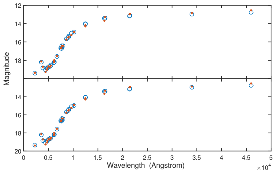
Figure 5: Standardised photometric measurements (dots) compared with predicted magnitudes (open circles) using the Table 4 parameters. The top panel results assume zero reddening, while the bottom panel is based on E(B - V) = 0.1 mag.
