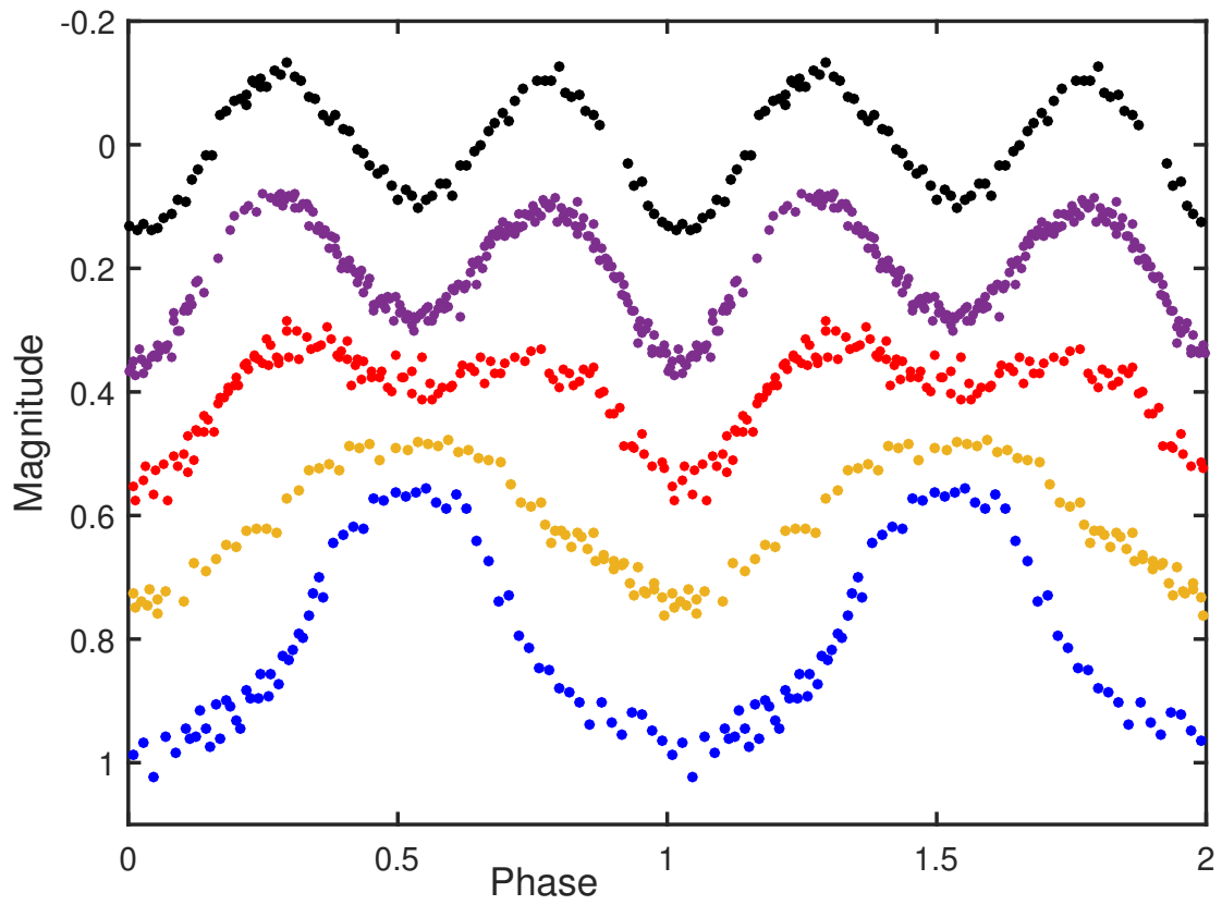
Figure 1: Phase-folded light curves of WISE 1526-113 obtained at SAAO. From top to bottom z , I , R , V and B . Zeropoints are arbitrary.
