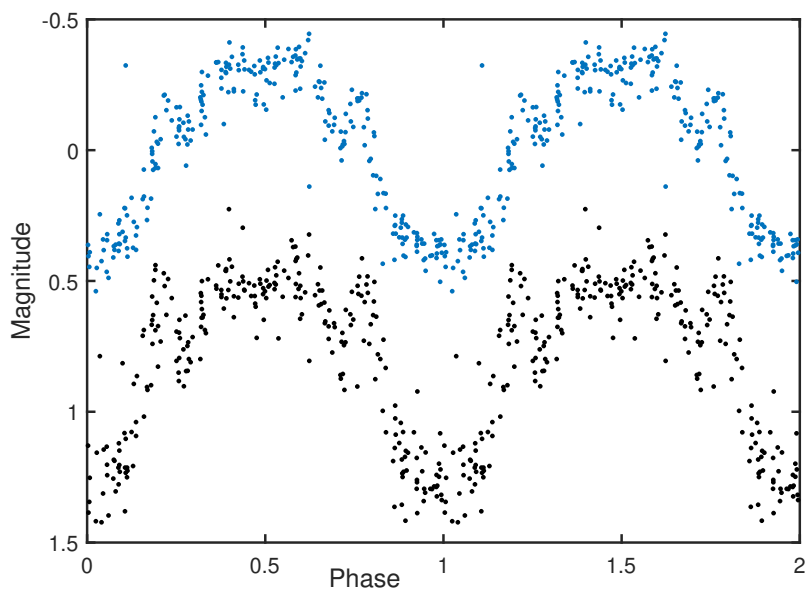
Figure 4: Phased WISE W1 (top) and W2 (bottom) light curves of WISE 1526-1113. Zeropoints are arbitrary.
