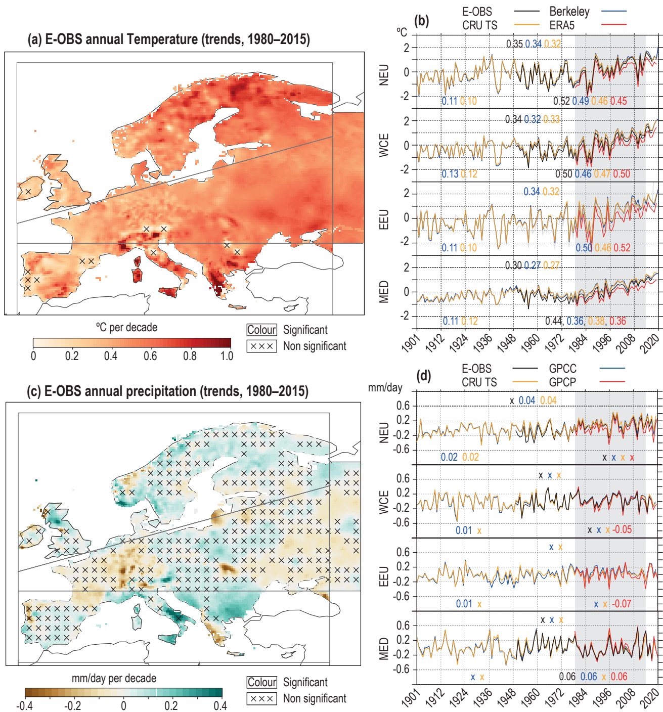
Figure Atlas.23 | (a) Mean 1980–2015 trend of annual mean surface air temperature (°C per decade) from E-OBS (Cortes et al., 2018). Data for non-European countries in the MED area are masked out. (b) Time series of mean annual temperature anomaly relative to the 1980–2015 period (shown with grey shading) aggregated for the land area in each of the four European sub-regions, from E-OBS, CRU, Berkeley and ERA5 (see Atlas.1.4.1 for description of global datasets). Mean trends for 1901–2015, 1961–2015 and 1980–2015 are shown for each dataset in corresponding colours in the same units as panel (a) (see legend in upper panel). (c) As panel (a) for annual mean precipitation (mm day -1 per decade). (d) As panel (b) for annual mean precipitation, from datasets E-OBS, CRU, GPCC and GPCP. Note that E-OBS data are not shown in panels (b) and (d) for the region EEU. For the MED region data are aggregated over the European countries alone. Trends have been calculated using ordinary least squares regression and the crosses indicate non-significant trend values (at the 0.1 level) following the method of Santer et al. (2008) to account for serial correlation. Further details on data sources and processing are available in the chapter data table (Table Atlas.SM.15).
