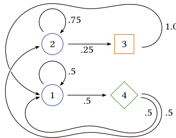
Figure 1: An example that does not satisfy Ad: a direct computation shows that [\circ \circ \dots \diamond] is too unlikely compared to [\circ \circ \dots \circ] .
